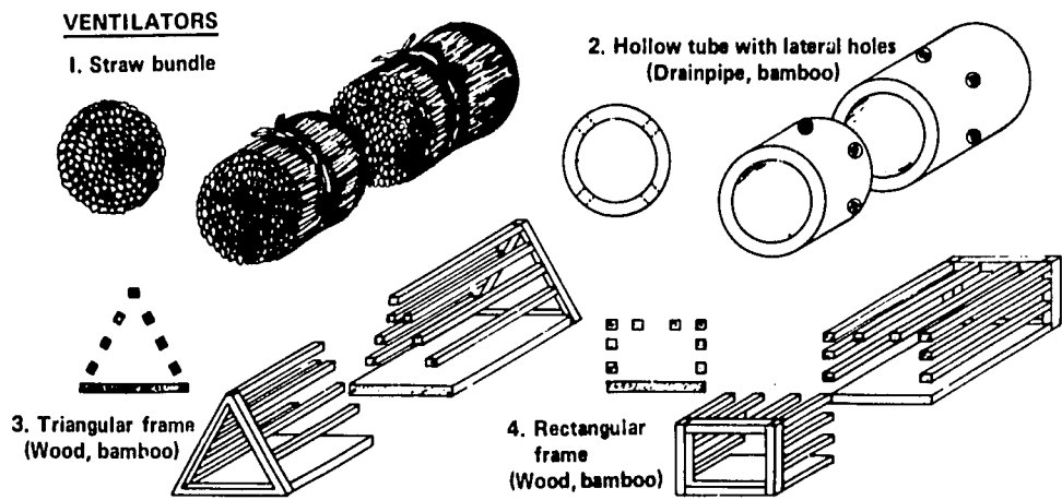
Figure 6. Design of cassava storage clamps.
