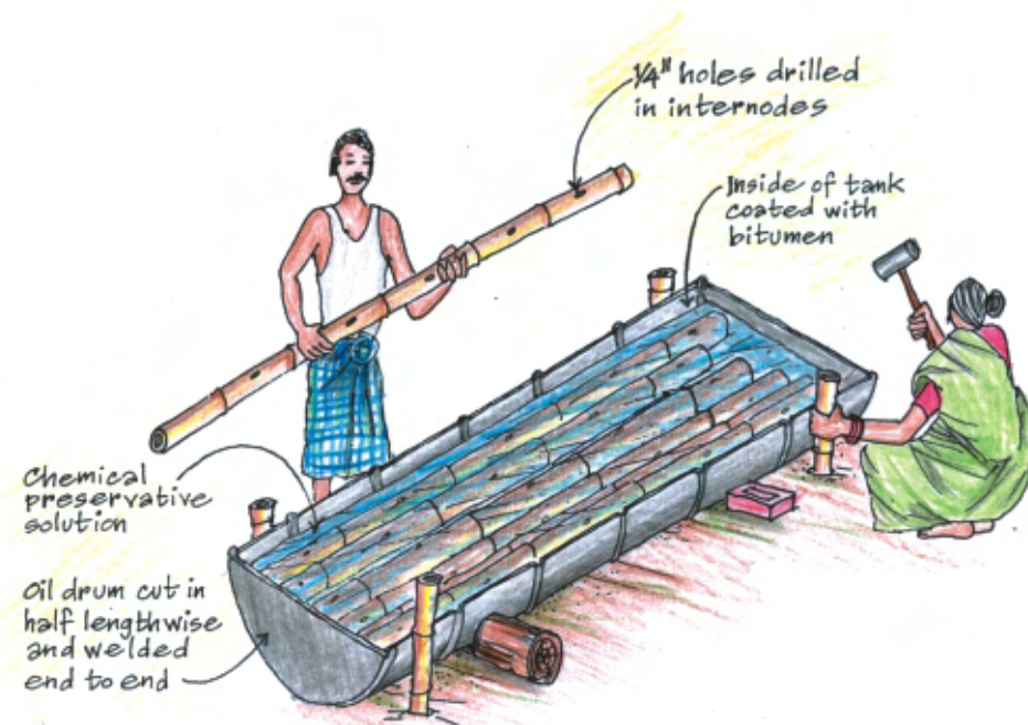
Fig. 3.3 Dip diffusion treatment of whole bamboo culms (adapted from: NMBA 2004)
