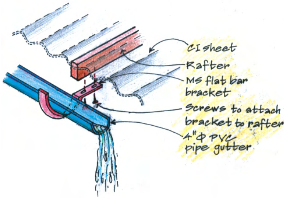
Fig. 2.13 PVC pipe rainwater gutter detail and house being built with a gutter
