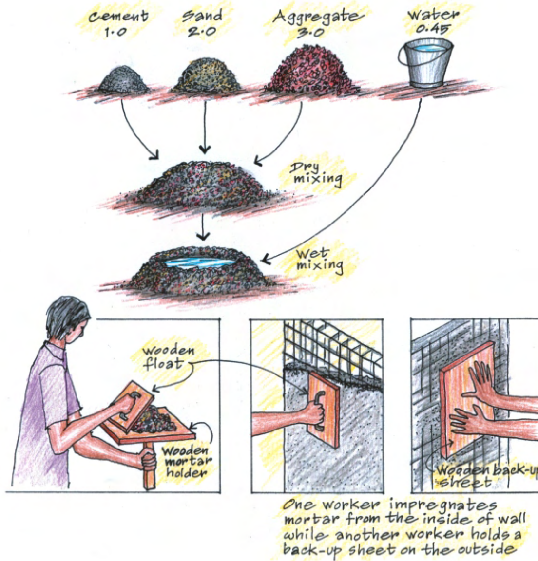
Fig. 5.6 Ferrocement construction process (adapted from Sharma and Gopalratnam 1980)
