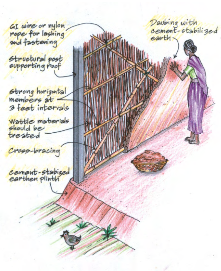
Fig. 4.3 Guidelines for wattle-and-daub construction
