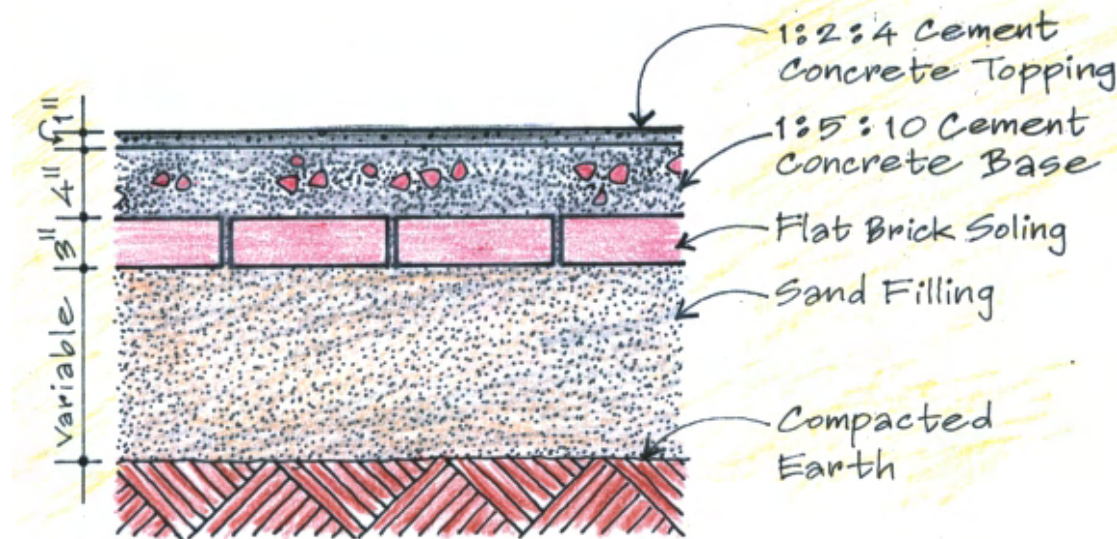
Fig. 2.3 Cement concrete flooring detail and house with cement concrete plinth
