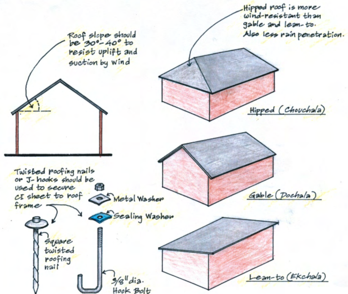
Fig. 2.12 Basic features of wind-resistant roofing (adapted from Mayo 1988)
