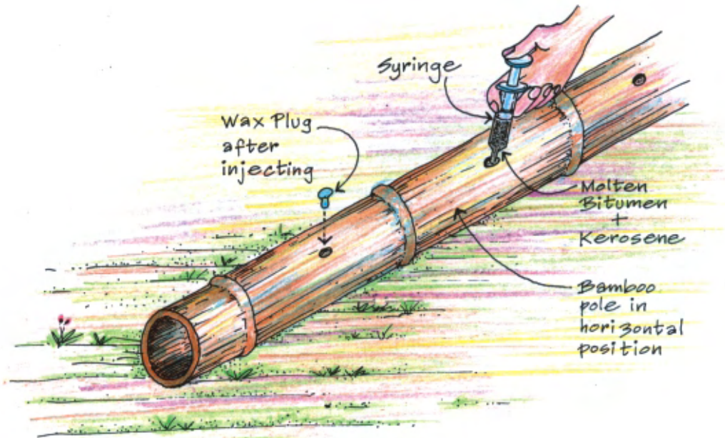
Fig. 3.4 Internodal injection method for treatment of whole bamboo culm
