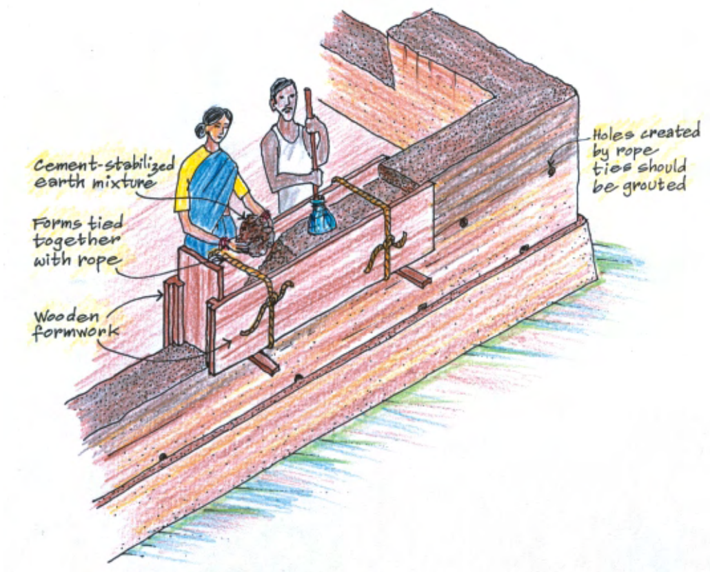
Fig. 4.7 House being built in Dinajpur using the rammed earth method and construction process of rammed earth wall
