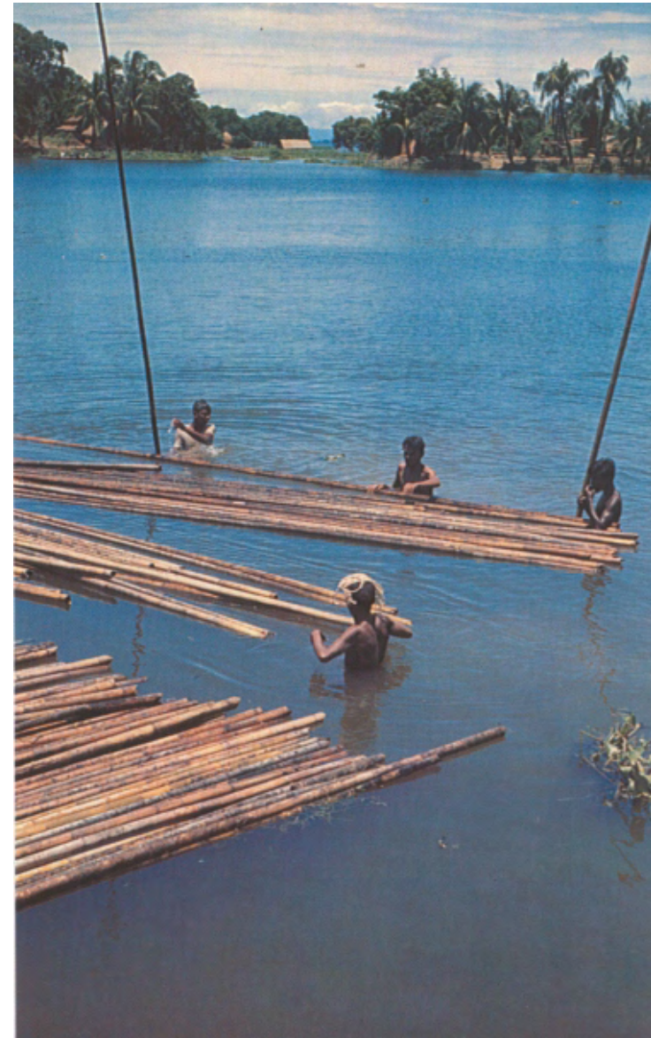
Fig. 3.2 Bamboo treatment by soaking in water (“pynot”) (photo: Barker 1994)
