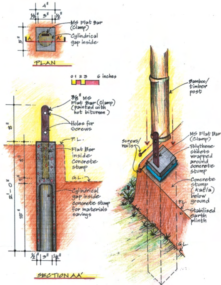
Fig. 5.1 Details of hollow kaatla and its production
