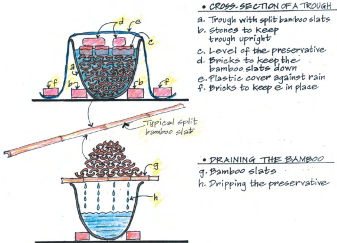
Fig. 2.8 Bamboo treatment by soaking in chemical preservatives (adapted from Janssen 1995)
