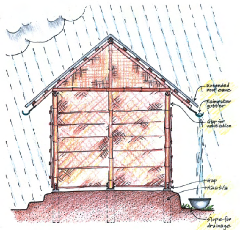
Fig. 3.6 Design aspects of building a bamboo house
