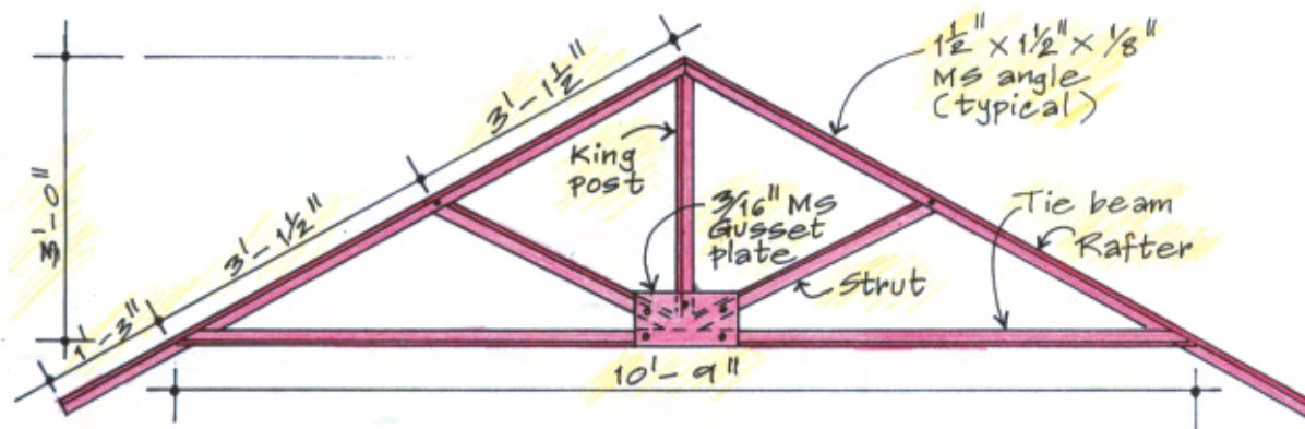
Fig. 5.8 MS angle roof truss used by Caritas (adapted from Caritas) and house with MS angle truss built by Proshika
