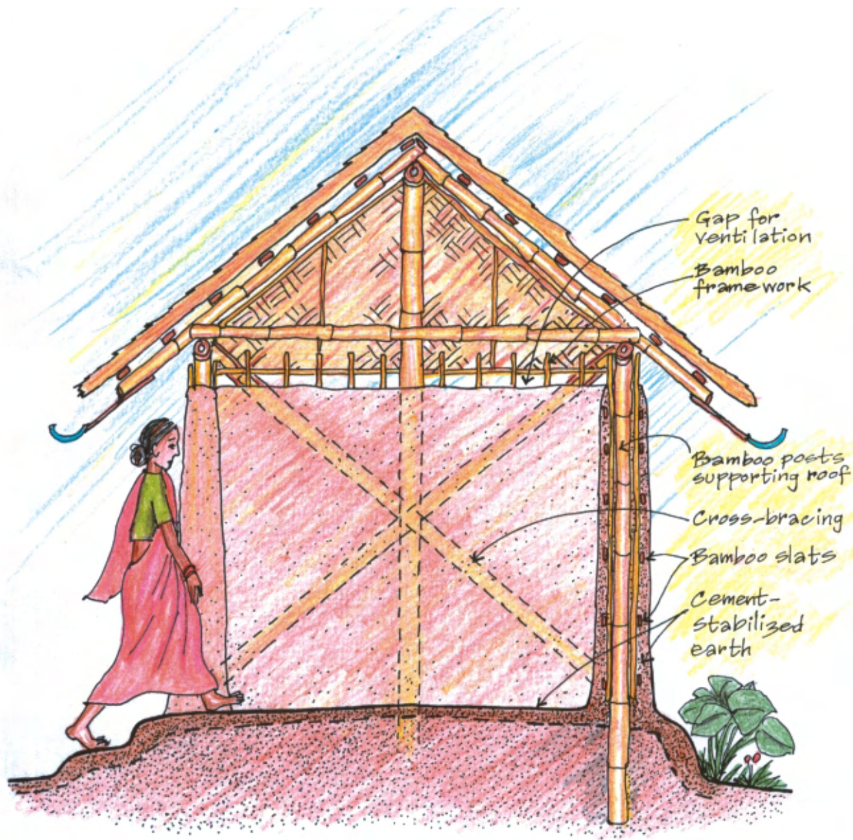
Fig. 4.8 Design aspects of building an earthen house
