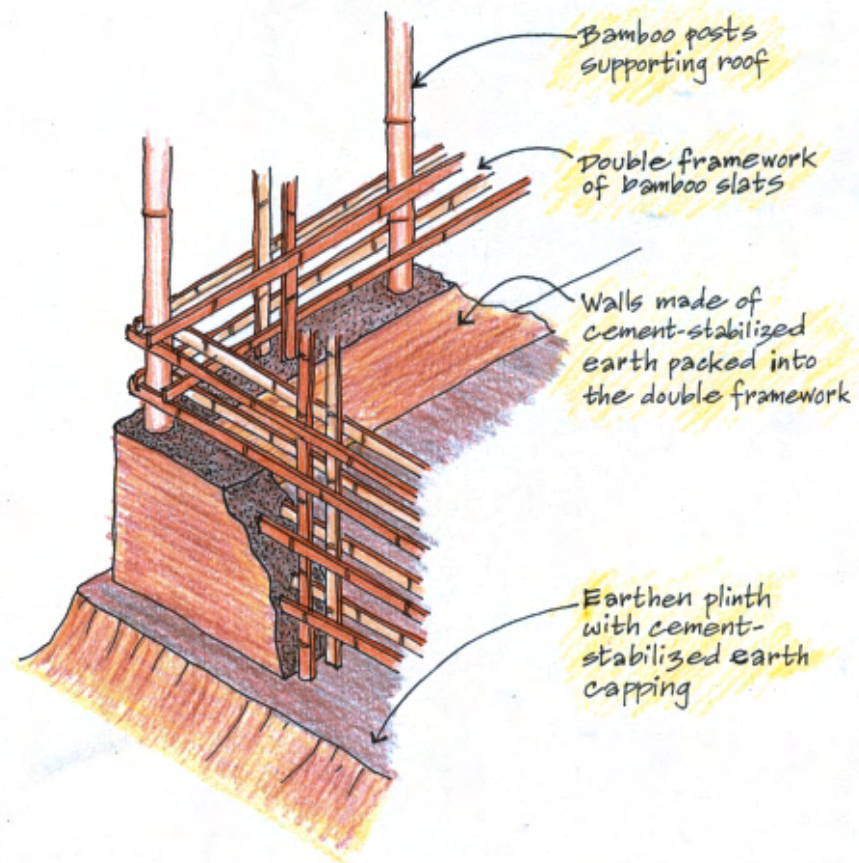
Fig. 4.4 Construction of wall with double layer framework and earth infill (adapted from Norton 1986)
