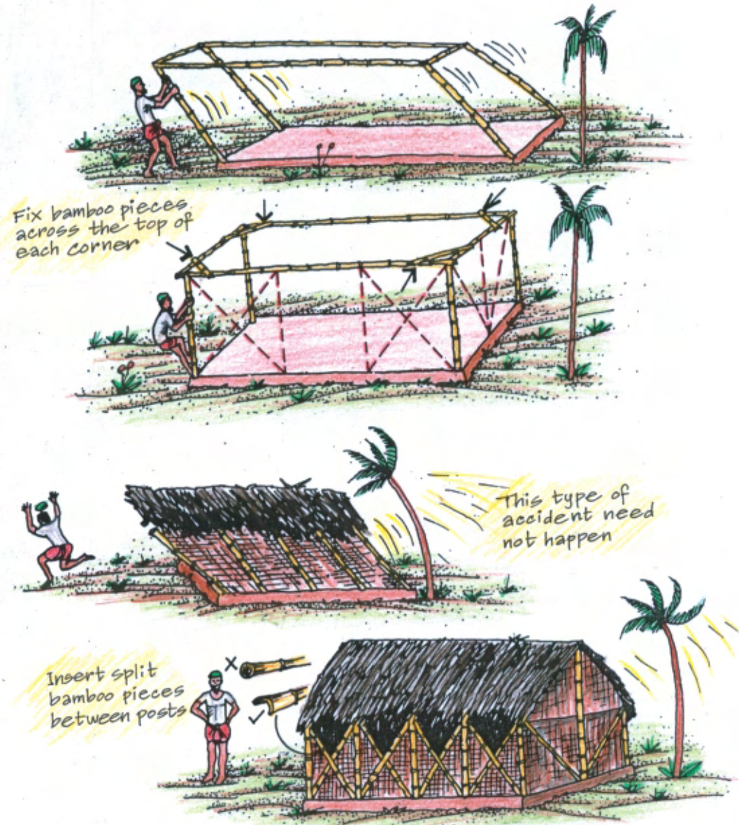
Fig. 2.9 Cross-bracing of bamboo structural frame (adapted from Chisholm 1979)
