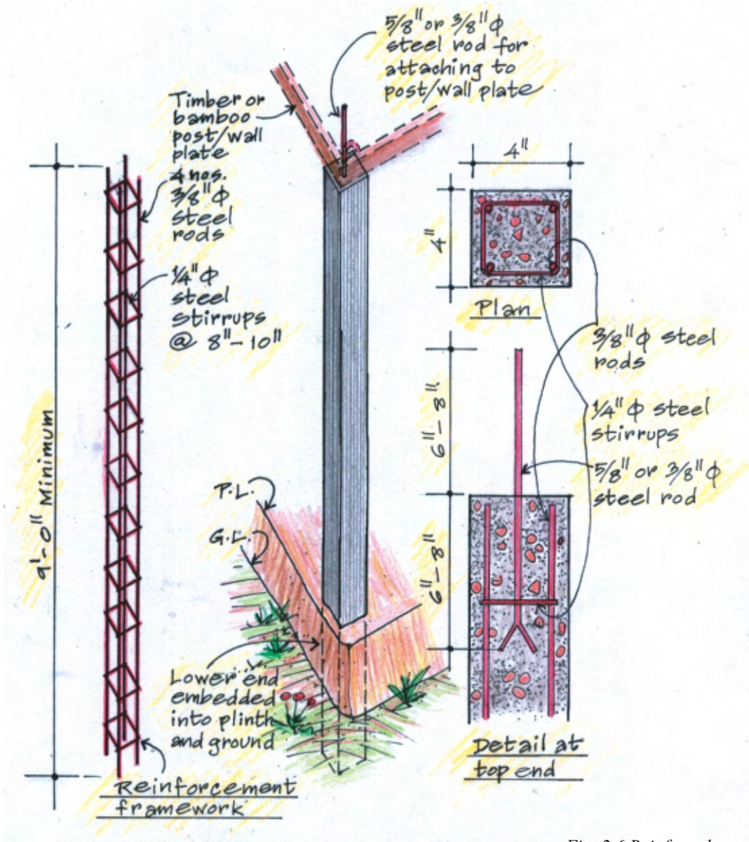
Fig. 2.6 Reinforced concrete post
