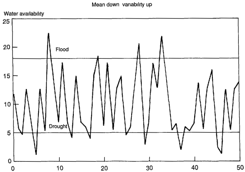
4 Mean water availability decreases and variability increases. The frequency and severity of drought have increased dramatically; the frequency of floods has increased slightly because of the increased variability.
