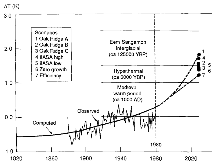
3 Simulation of temperature response to CO 2 effect only Calculation from 1820 to 2030 with a parameterized form of a 1 D radiative convective model for the atmosphere (Hansen 1983) coupled to a 1 D energy balance model for the ocean (Cess and Goldenberg 1981) Observed temperature for the Northern Hemisphere from 1880 to 1980 (Jones et al 1982) Reference period 1946-60
