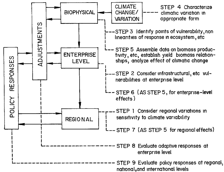
5 Causal (top down) and adjoint (bottom up) methods for climate impact assessment. The adjoint approach was adopted in the IIASA/UNEP project (Parry and Carter 1988)
