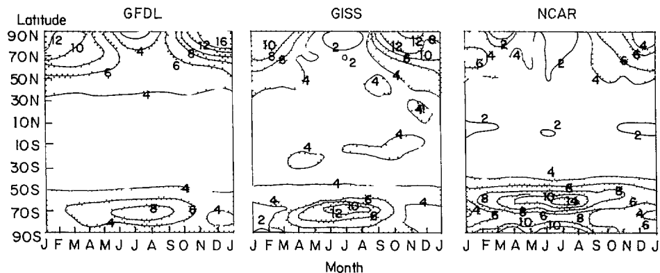
4 Latitude time cross section of the zonal mean surface air temperature change ( ^{\circ}\text{C} ) for a doubling of the atmospheric \text{CO}_2 concentration simulated by the global climate models of GFDL GISS and NCAR. Stippling indicates temperature increases greater than 4^{\circ}\text{C} (From Schlesinger and Mitchell 1985 Fig 4.40)
