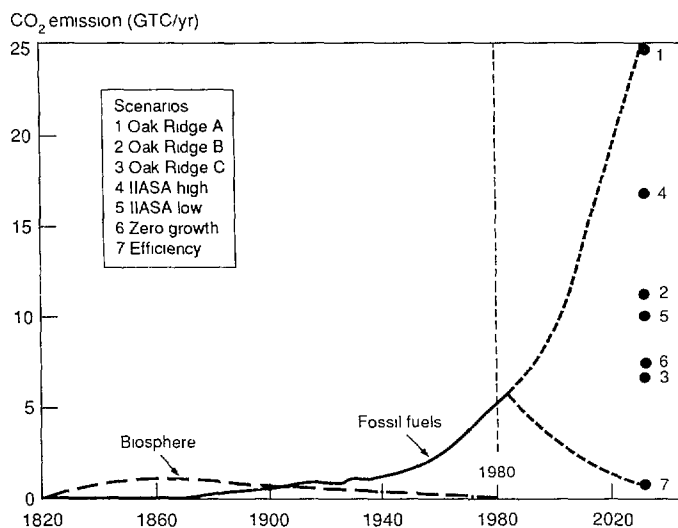
1 Simulation of CO 2 emission. The historical development is based on biospheric sources from 1820 to 1980 and on U N statistics for fossil fuel use, cement production, and gas flaring from 1860 to 1980. The projection from 1980 to 2030 is based on the specifics of the listed energy scenarios (Bach 1986).
