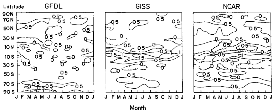
5 Latitude time cross section of the zonal mean precipitation rate change (mm/d) for a doubling of the atmospheric \text{CO}_2 concentration simulated with the global climate models of GFDL GISS and NCAR. Stippling indicates a decrease in precipitation rates (From Schlesinger and Mitchell 1985 Fig 4.43)
