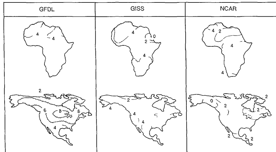
1 Distribution of surface air temperature change (°C) for a doubling of atmospheric CO 2 concentration for June, July, and August simulated by the global climate models of GFDL, GISS, and NCAR. Stippling indicates temperature increases greater than 4 °C (Redrawn from Fig. 4.39 of Schlesinger and Mitchell 1985).
