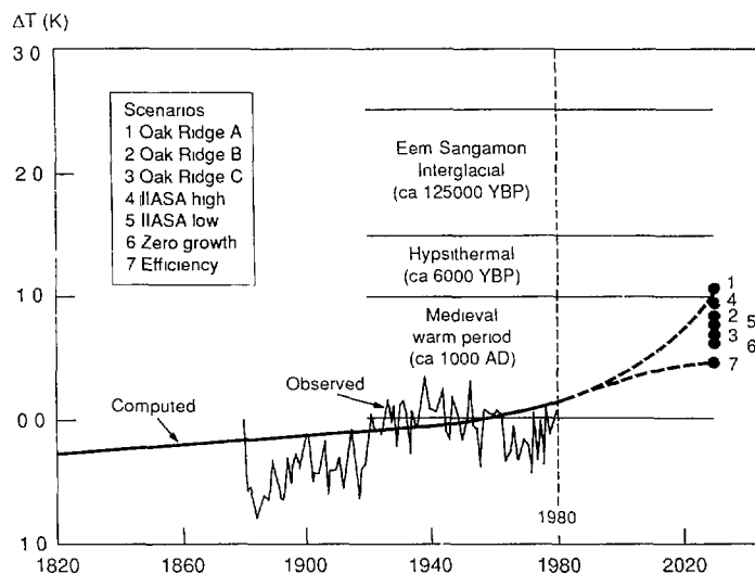
4 Simulation of temperature response to the combined effects of CO 2 and other GHG (CH 4 , N 2 O, CFC-11 and 12)
