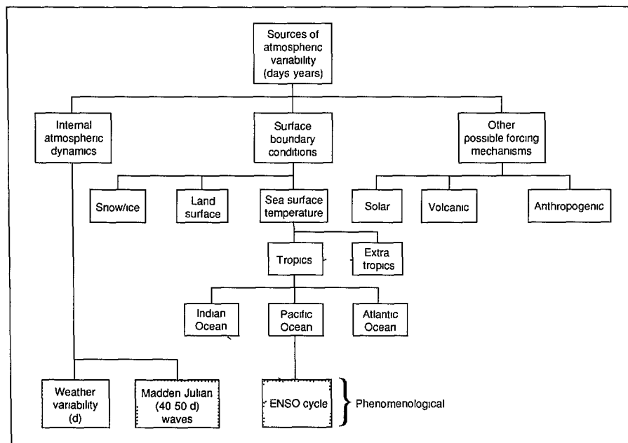
1 Schematic illustration of the causes of atmospheric variability on time scales ranging from days to years. The bottom tier of boxes represents selected phenomenological aspects of variability; two of them (shaded boxes) are discussed here.
