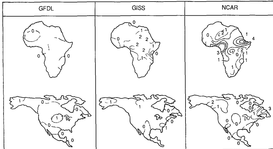
2 Distribution of precipitation rate change (mm/d) for a doubling of atmospheric CO 2 concentration for June July and August simulated by the global climate models of GFDL GISS and NCAR Stippling indicates a decrease in precipitation rate (Redrawn from Fig 4 42 of Schlesinger and Mitchell 1985)
