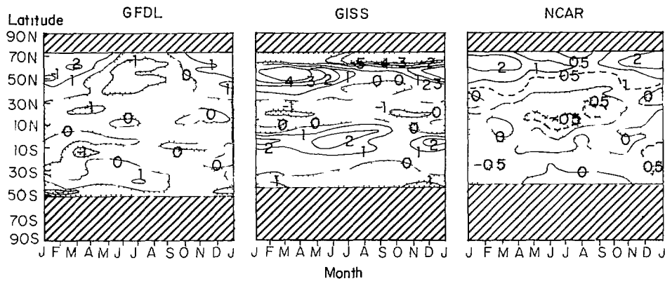
6 Latitude time cross section of zonal mean soil water content change (cm) over ice free land for a doubling of the atmospheric CO 2 concentration simulated with the global climate models of GFDL, GISS and NCAR. Stippling indicates a decrease in soil water; hatching indicates latitudes where there is no ice free land (From Schlesinger and Mitchell 1985, Fig. 4.46)
