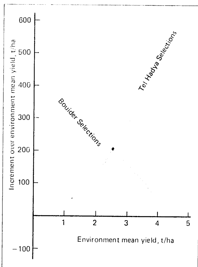
Figure 2. Select under stress for performance under stress. Tel Hadya is a reasonably favored site with an average annual rainfall of 330 mm, whereas Bouider receives only 180 mm. Points on the scale Environment mean yield are obtained by taking the average yield of 155 barley genotypes in one season at one site; thus this scale can be read as an indicator that is inversely proportional to stress. Points on the scale Increment over environment mean yield are for selected genotypes in the same seasons at the same sites. The regression line labelled Tel Hadya Selections is based on the average yield of 29 genotypes that had been selected at Tel Hadya for performance superior to that of the local check Arabi Abiad . The regression line labelled Bouider Selections is based on the average yield of 15 genotypes selected at Bouider for performance superior to Arabi Aswad .
