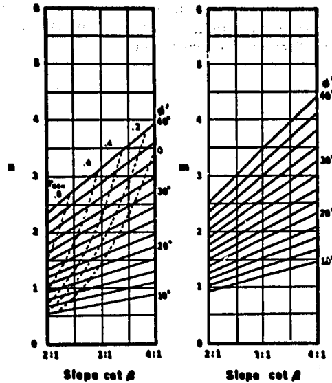
Figure 5. Stability coefficients, m and n , for \frac{c'}{\gamma H} = 0.05 and D = 1.00 [after Bishop and Morgenstern (2)].
