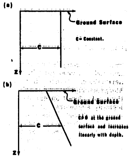
Figure 1. Comparison of assumptions for cohesion, c , as made by various investigators.
