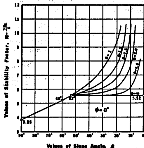
Figure 3. Relations between slope angle, \beta , and stability number, N , for different values of depth factor, D [after Terzaghi and Peck (11)].
