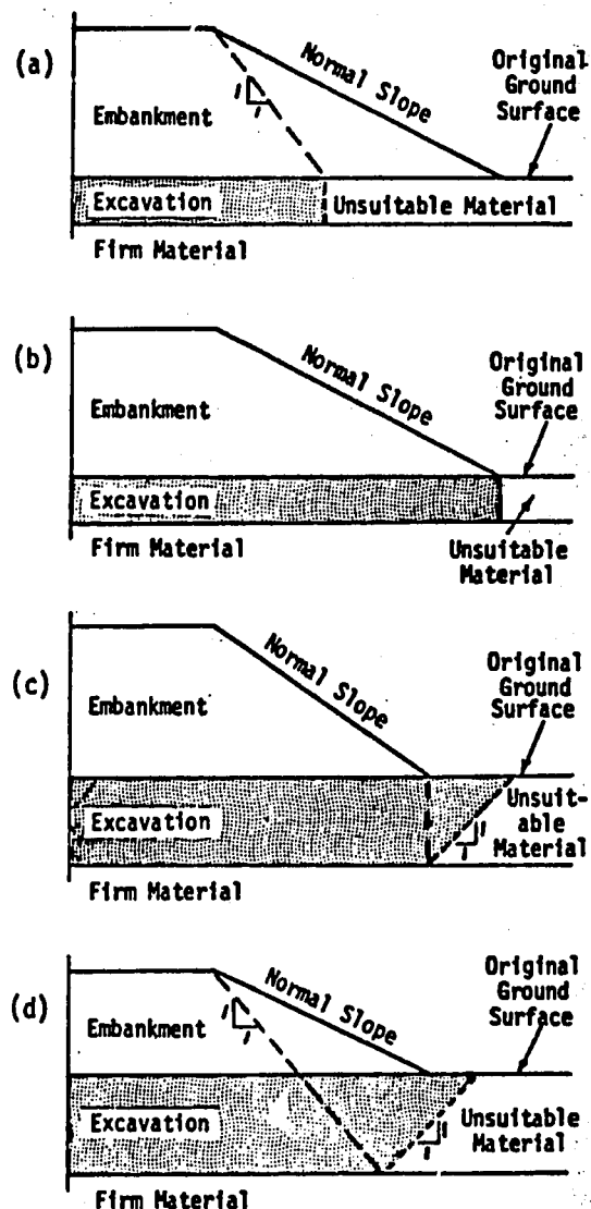
Figure 5. Examples of excavation of unsuitable material.
