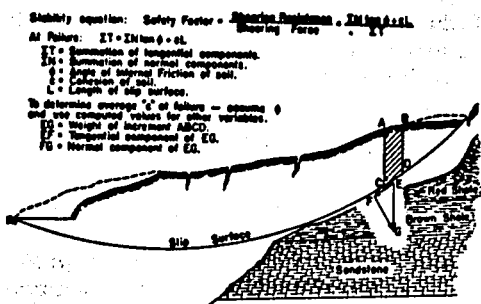
Figure 10. Solution by graphical integration. The total area is divided into increments of the same width as ABCD. Weight of the soil is computed and graphically resolved into its tangential and normal components.
