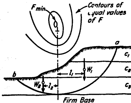
Fig. 35.5. Base failure in stratified cohesive soil.
