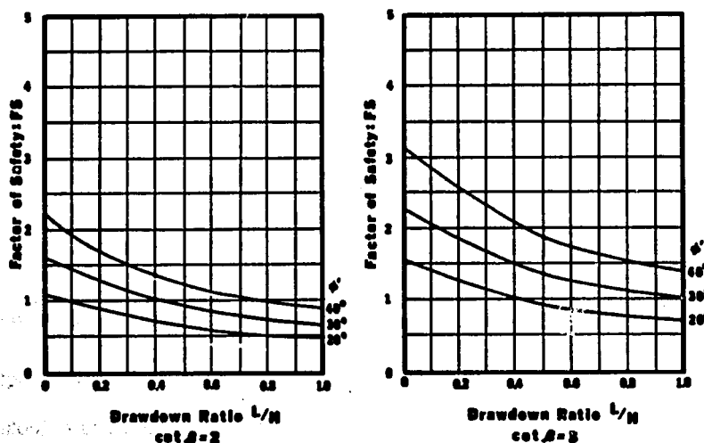
Figure 8. Relationship between factor of safety, FS, and drawdown ratio, L/H , for \frac{c'}{\gamma H} = 0.0125 [after Morgenstern (6)].
