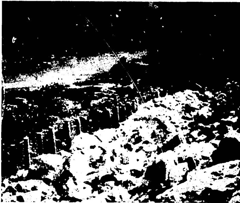
Fig. 51 Boulders placed at toe of sliding mass to supplement piling
