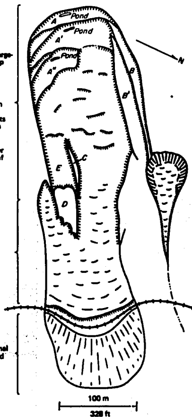
Figure 2.10. Ames slide near Tellurido, Colorado (2.182, 2.183). This slump-earth flow landslide occurred in glacial till overlying Mancos shale. Repeated slumping took place along upper margins after main body of material had moved down. Long axes of slump blocks B and B' are parallel with rather than perpendicular to direction of movement of main part of slide. Blocks B and B' moved toward left, rather than toward observer.
