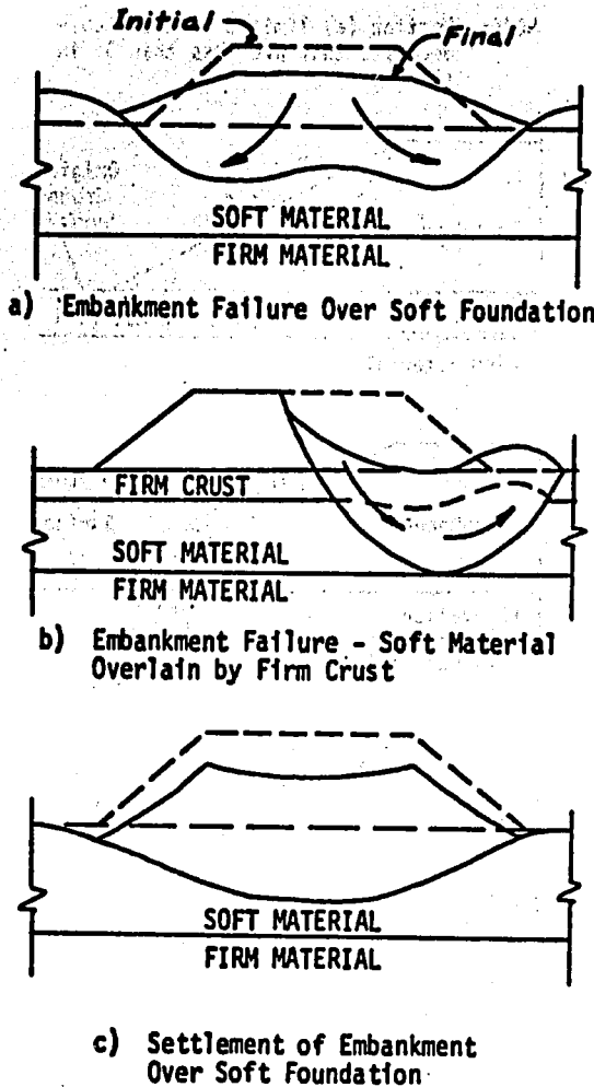
Figure 4. Typical embankment problems over soft foundations.
