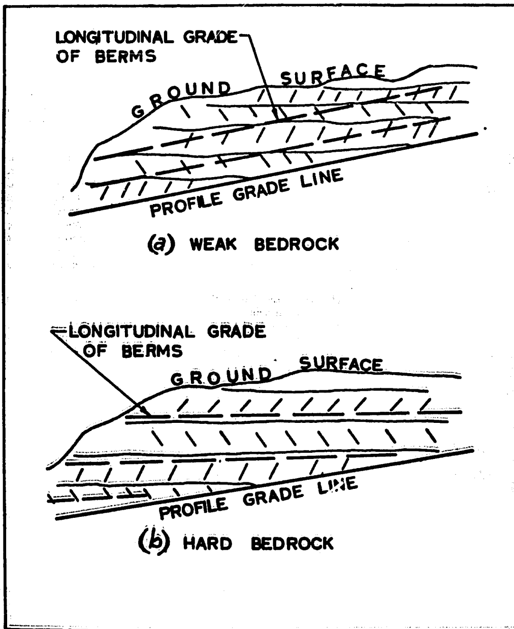
Fig. 21 Longitudinal grade for bedrock berms
