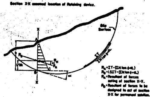
Figure 14. Method for computing the forces acting at a given point in a slide. The value of T and N is determined for the area desired (from X-X to top in this sketch). The difference between the forces causing movement ( \sum T ) and the resistance to movement ( \sum N \tan \phi + cL ) is designated as R_A . The resistance that will produce a safety factor of 1.5 is designated as R_D .
