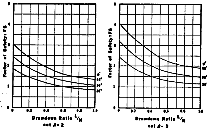
Figure 10. Relationship between factor of safety, FS, and drawdown ratio, L/H, for \frac{c'}{\gamma H} = 0.050 [after Morgenstern (8)].
