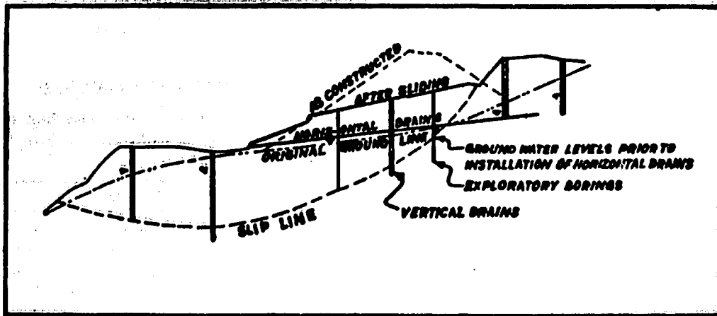
Fig. 90 Slide treatment consisting of horizontal drains and vertical drain wells. (Courtesy of California Division of Highways)
