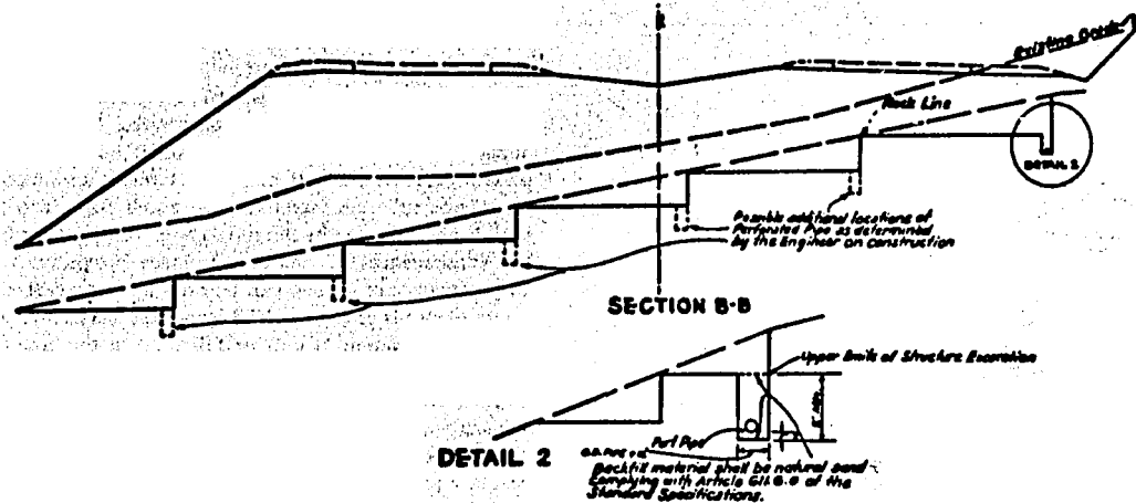
Figure 10. Typical detail for longitudinal underdrain.
