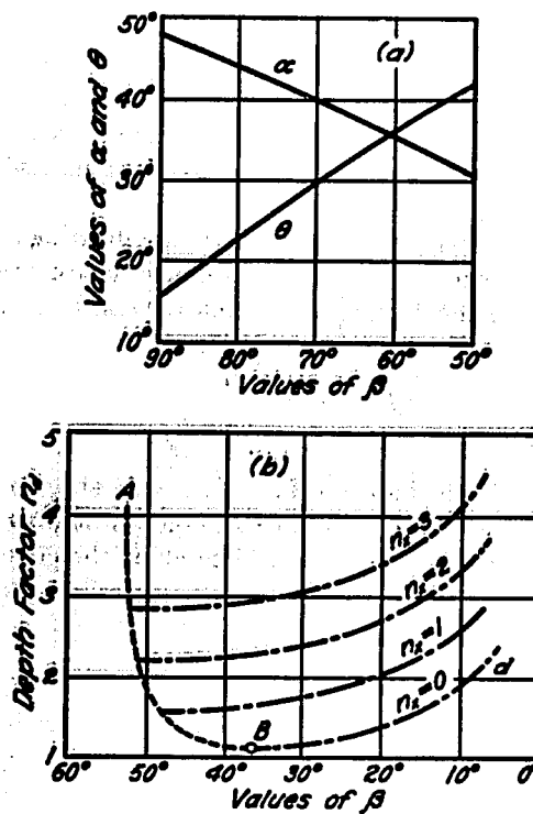
Fig. 35.4. (a) Relation between slope angle \beta and parameters \alpha and \theta for location of critical toe circle when \beta is greater than 53^\circ . (b) Relation between slope angle \beta and depth factor n_s for various values of parameter n_d . (after W. Fellenius 1927).
