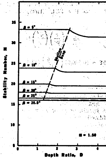
Figure 14. Relationship between depth factor, D , and stability number, N , for \phi = 0 for selected values of slope inclination [from Hunter and Schuster (4)].
