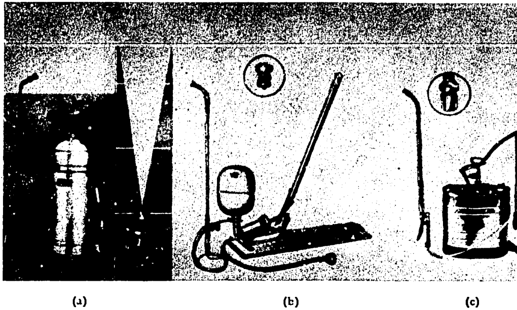
Fig. 47 (a) Hand compression sprayer with 3-action adjustable nozzle (b) Gator rocking sprayer with circular mist type nozzle (c) Knapsack sprayer with flat fan type nozzle
