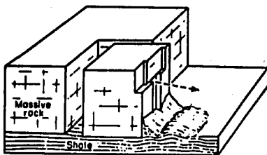
Figure 2.12. Block slide at quarry (2.182).
