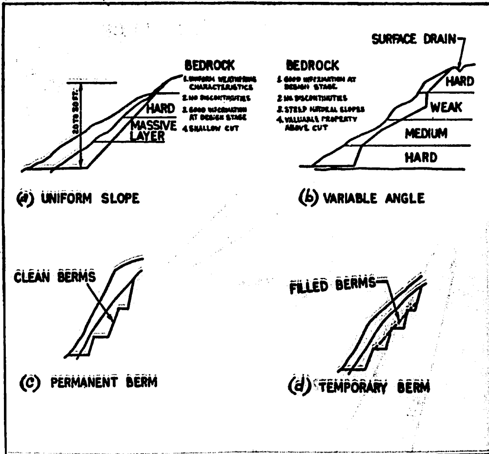
Fig. 20 Types of bedrock cut slopes
