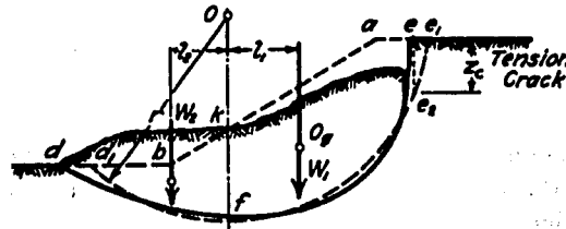
Fig. 35.1. Deformation associated with slope failure.
