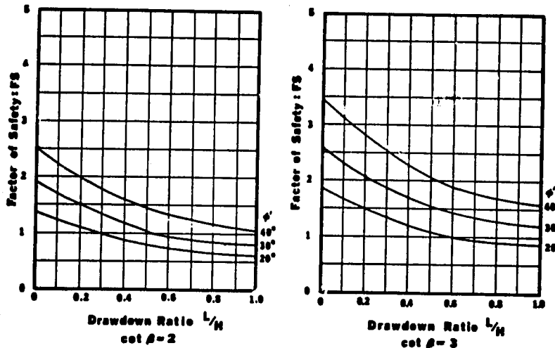
Figure 9. Relationship between factor of safety, FS, and drawdown ratio, L/H, for \frac{c'}{\gamma H} = 0.025 [after Morgenstern (6)].
