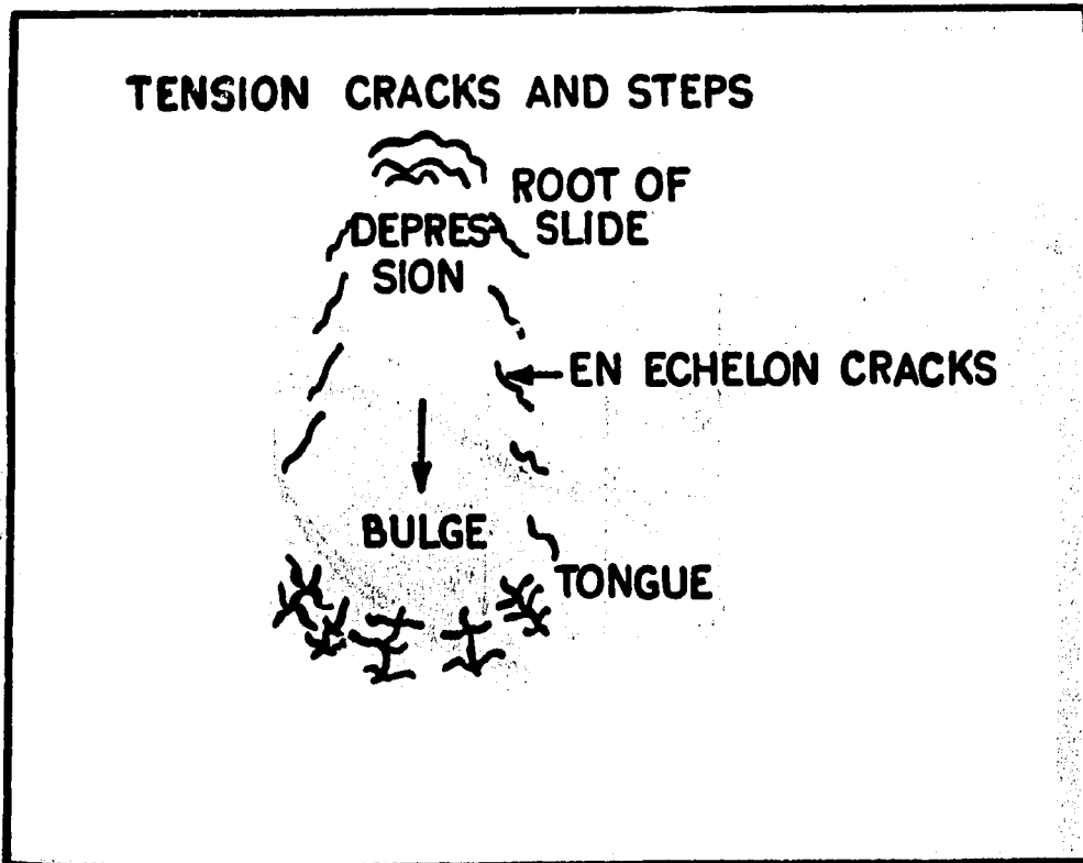
Fig. 27 Plan of typical slide in cohesive material
