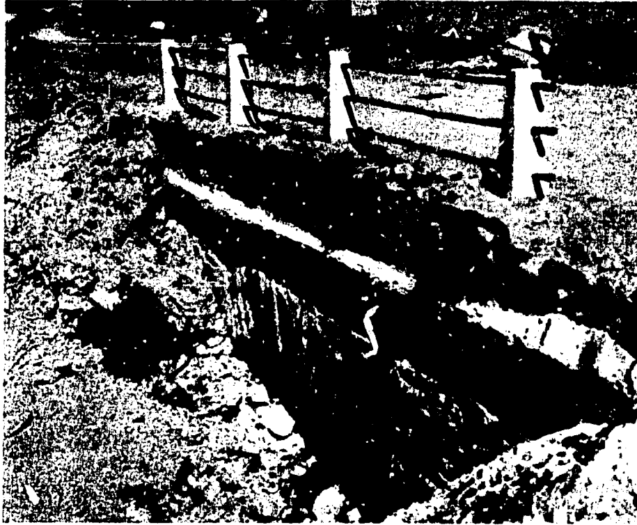
Fig. 36 Culverts clogged up due to poor maintenance practice
