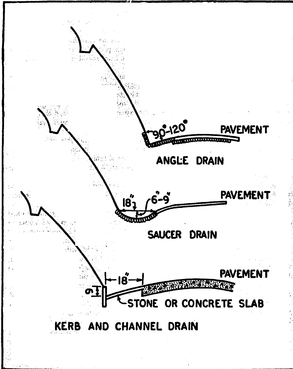
Fig. 58 Types of drains
