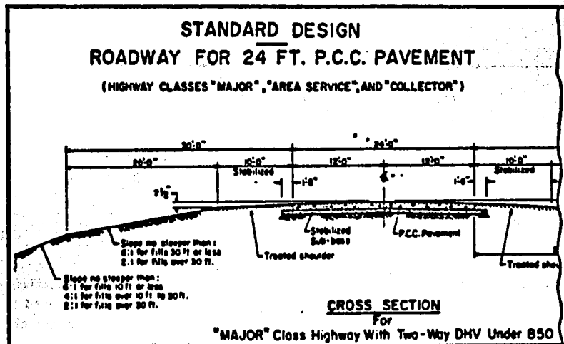
Figure 13. Typical standard design slopes.
