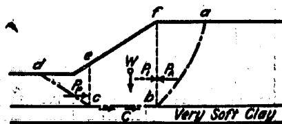
Fig. 35.13. Failure of slope underlain by thin layer of very soft clay.
