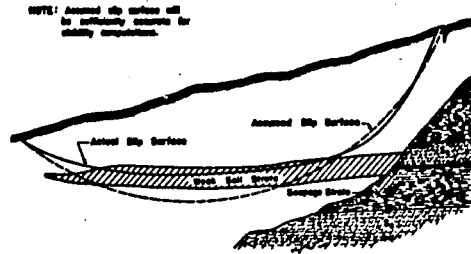
Figure 9. The presence of a weak soil layer will tend to produce a failure within its limits. On occasions, the actual slip-surface will be as close to the theoretical position indicated, and the circle can be used in the computations.
