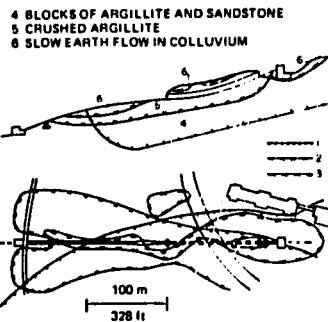
Figure 2.32. Three-storied landslide in Sochi on coast of Black Sea, USSR (2.173). Boundaries of three stories of sliding are shown in section and plan by three types of lines.
