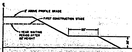
Figure 6. Typical embankment with berms and stage construction.
