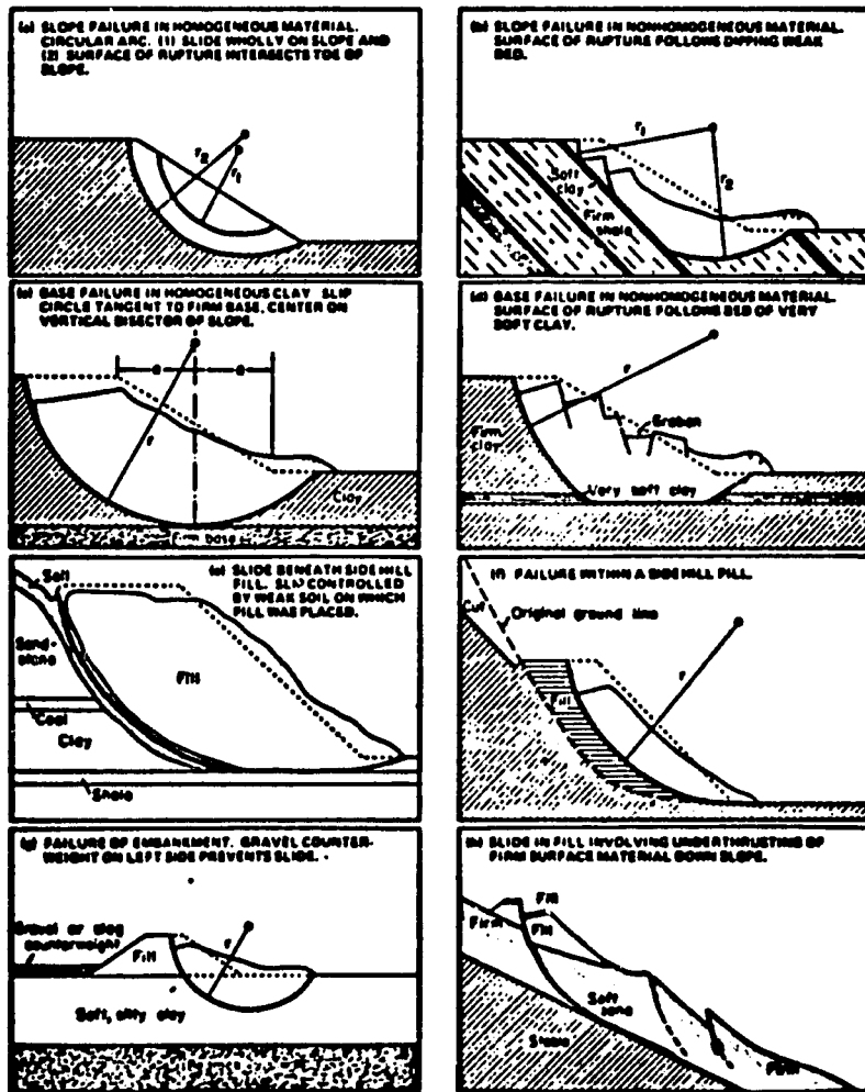
Figure 2.8. Varieties of slump (2.182).
