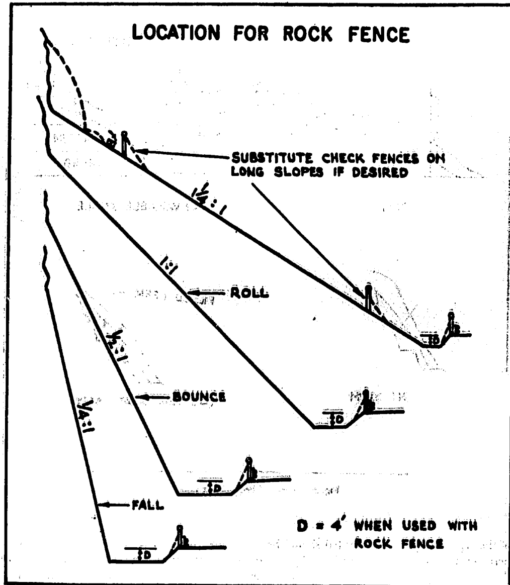
Fig. 19 Position of installation of rock fence used either as check fence on slope or as protection on highway. Though ditch design for \frac{3}{4} :1 and \frac{1}{2} :1 for a 100 ft. high slope is same, yet rock \frac{3}{4} :1 slope must cover a greater distance before encountering same fence
