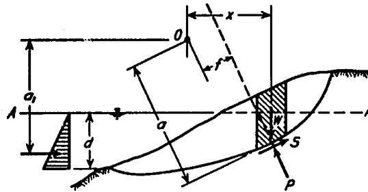
Fig. 35.10. Geometry of method of slices for investigating equilibrium of slope if surface of sliding is not circular.
