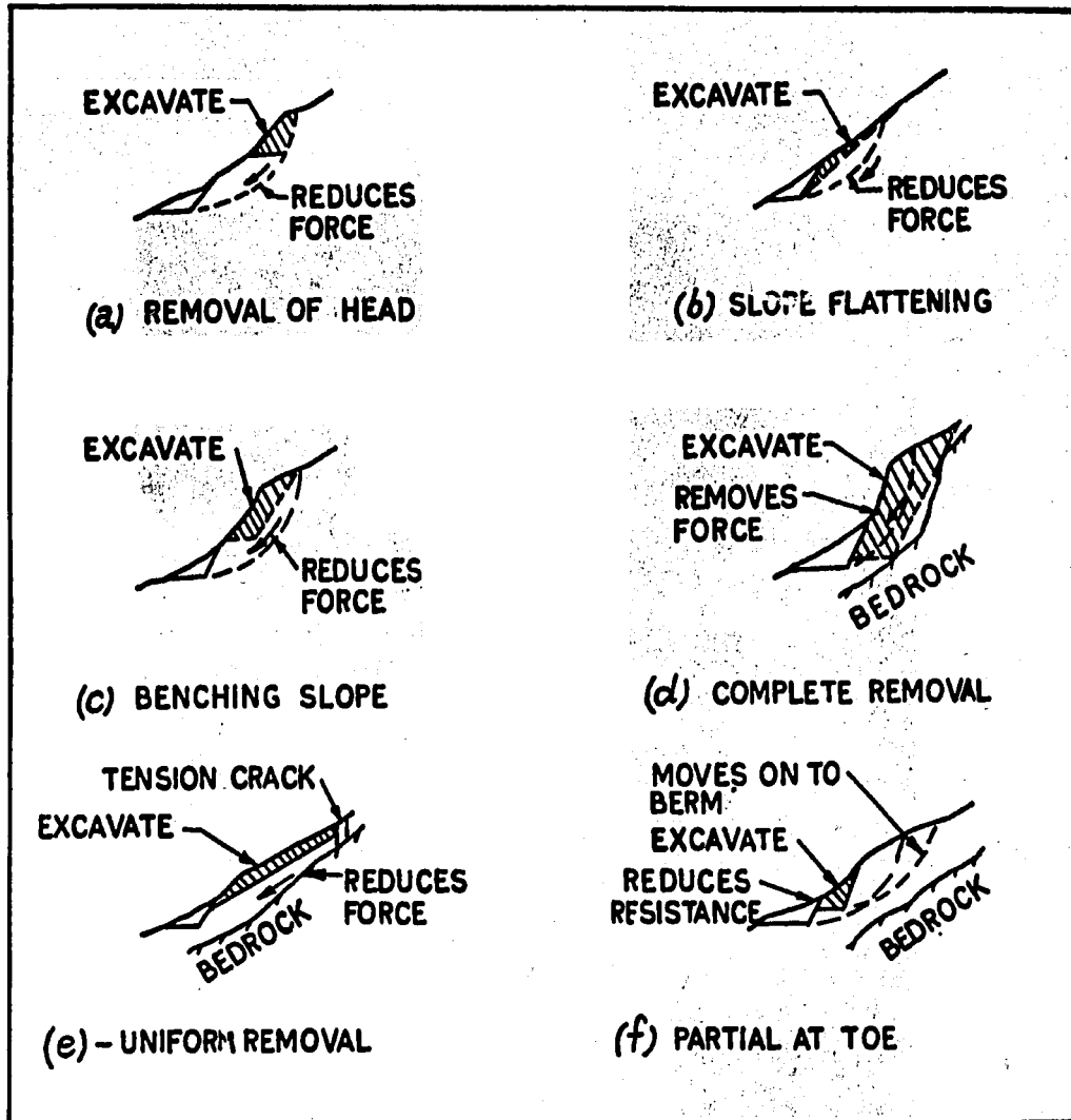
Fig. 34 Excavation techniques
