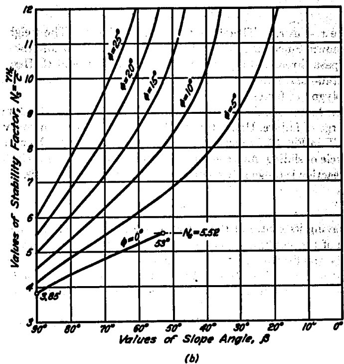
Fig. 35.6. Failure of slope in material having cohesion and friction. (a) Diagram illustrating friction-circle method. (b) Relation between slope angle \beta and stability factor N_s for various values of \phi (after Taylor 1937).
