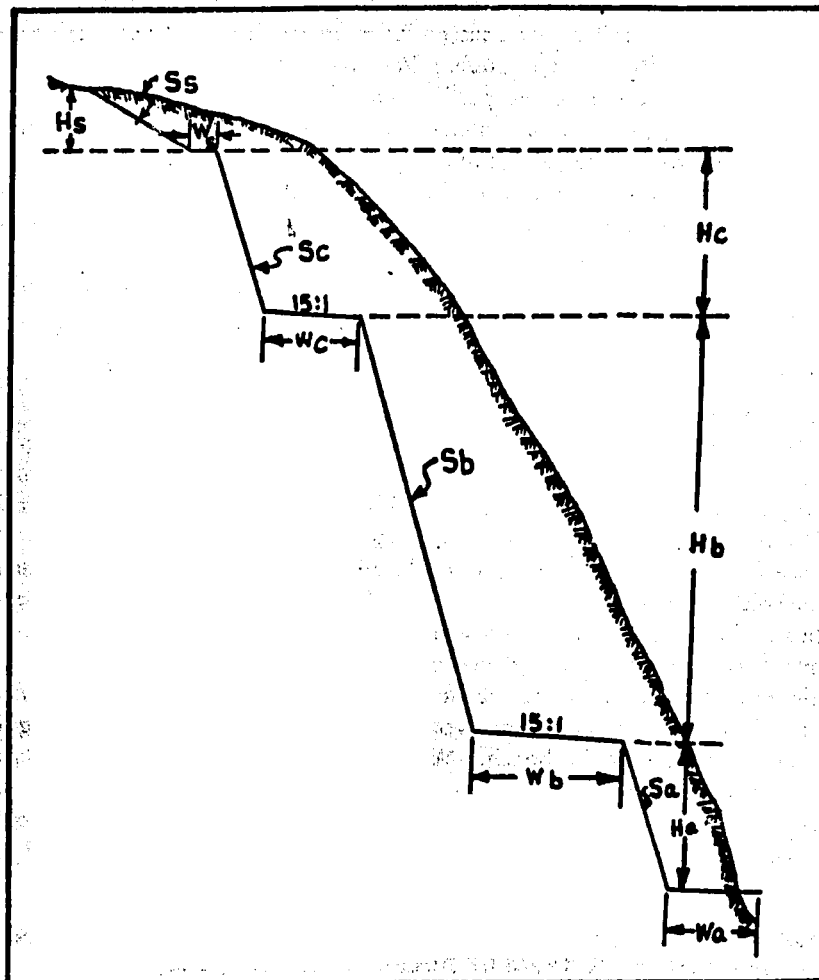
Fig. 35 Criteria for bed rock slope design as used by West Virginia State Road Commission. This technique employs a combination of benches and relative steep back slopes (Refer to Table 7)
