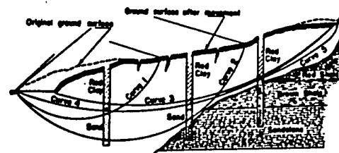
Curves 1,2,3,4, and 5 represent potential slip planes.
