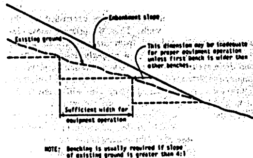
Figure 7. Cross section of typical longitudinal benches.
