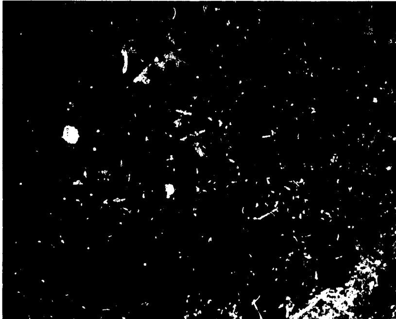
Fig. 45 Condition of slope after treatment (asphalt mulch technique)
