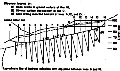
Figure 13. Cross-section of the slide pictured in Figures 11 and 12. The slide has been divided into increments and the computation of \sum T and \sum N is given in Table 1.
