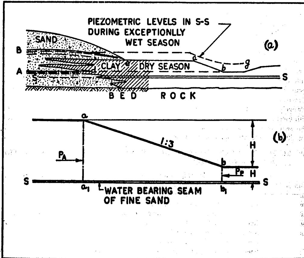
Fig. 24 (a) Geological conditions involving danger of slope failure by spreading. (b) Diagram of forces which act on soil beneath slope ab
