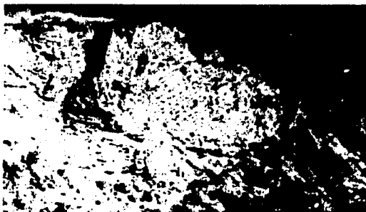
Figure 2.7. Slump in thinly bedded lake deposits of silt and clay in Columbia River valley (note backward tilting of beds above surface of rupture) (2.182).
