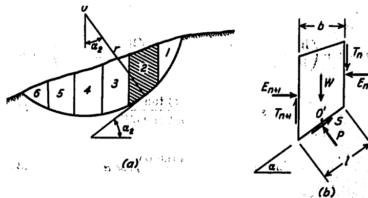
Fig. 35.7. Method of slices for investigating equilibrium of slope located above water table. (a) Geometry pertaining to one circular surface of sliding. (b) Forces on typical slice such as slice 2 in (a).
