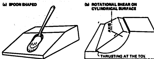
Figure 2.4. Slope failure in uniform material (2.182).
