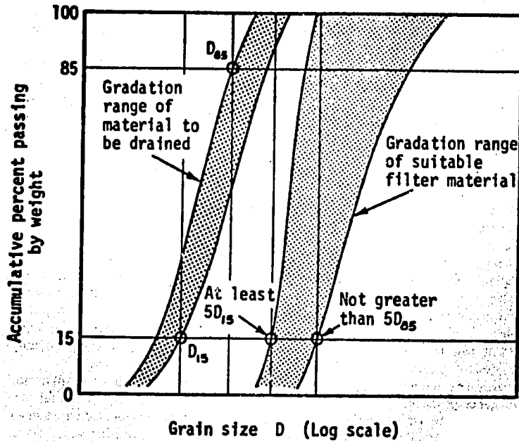
Figure 11. Typical gradation requirements for filters and pervious blankets.
