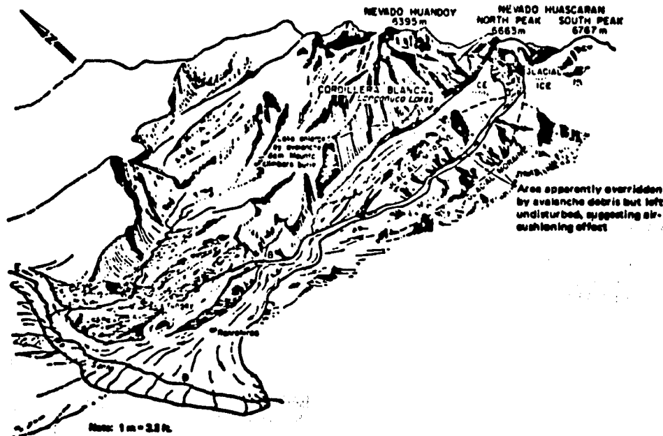
Figure 2.27. Area affected by May 31, 1970, Huascarán debris avalanche, which originated at point A (2.24). Yungay was protected from January 10, 1962, debris avalanche by 180 to 240-m (600 to 800-ft) high ridge (point B), but a portion of May 31, 1970, debris avalanche diverted from south side of canyon wall, topped "protective" ridge, and descended on Yungay below. Only safe place in Yungay was Cemetery Hill (point C), where some 93 people managed to run to before debris avalanche devastated surrounding area. Moving at average speed of 320 km (200 mph), debris arrived at point D, 14.5 km (9 miles) distant and 3660 m (12 000 ft) lower, within 3 to 4 min after starting from north peak of Huascarán. Debris flowed upstream along course of Rio Santa (point E) approximately 2.5 km (1.5 miles). Debris continued to follow course of Rio Santa downstream to Pacific Ocean, approximately 160 km (100 miles), devastating villages and crops occupying floodplain.
