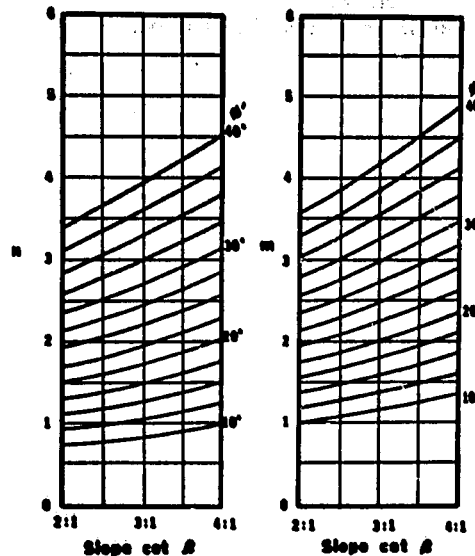
Figure 7. Stability coefficients, m and n , for \frac{c'}{\gamma H} = 0.06 and D = 1.50 [after Bishop and Morgenstern (2)].
