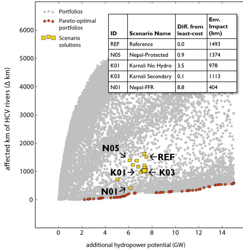
Figure 20: Least-cost environmental scenarios from the SWITCH energy options model evaluated in the SSP context
