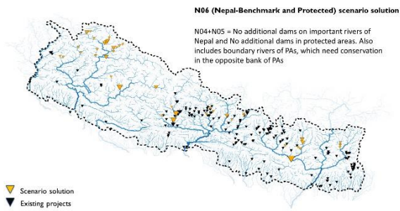
Figure 31. Portfolios resulting from the SWITCH energy model for the reference scenario and 13 environmental scenarios. For a description of the scenarios see 6.2.1.
