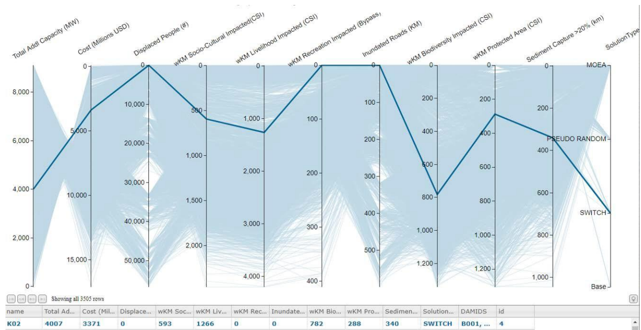
Figure 17: SWITCH least-cost solution for Scenario K02
