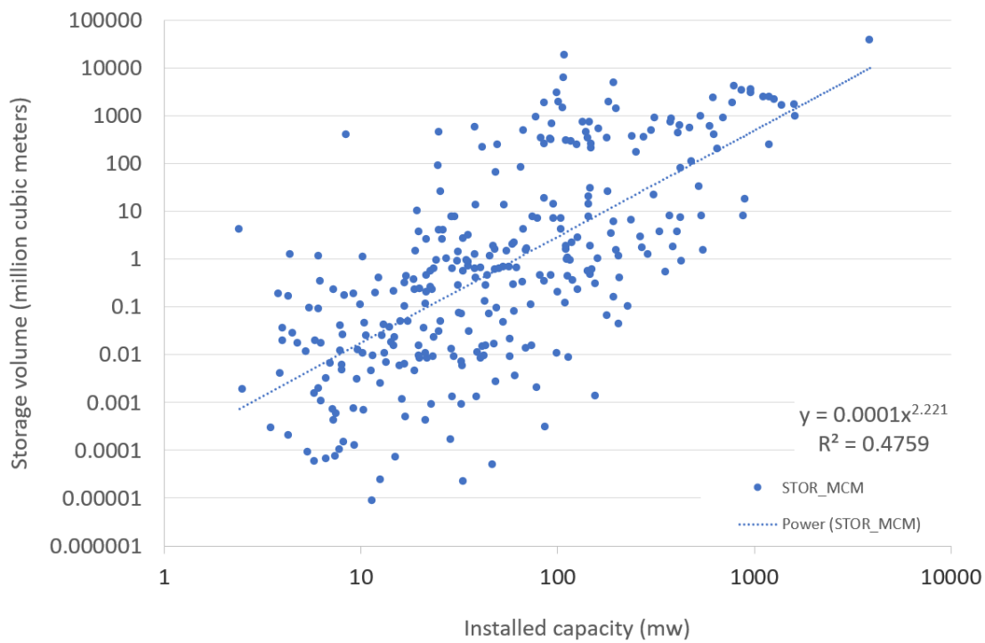
Figure 23: Estimation of storage volume using a power relationship based on data from Lahmeyer (2020)
