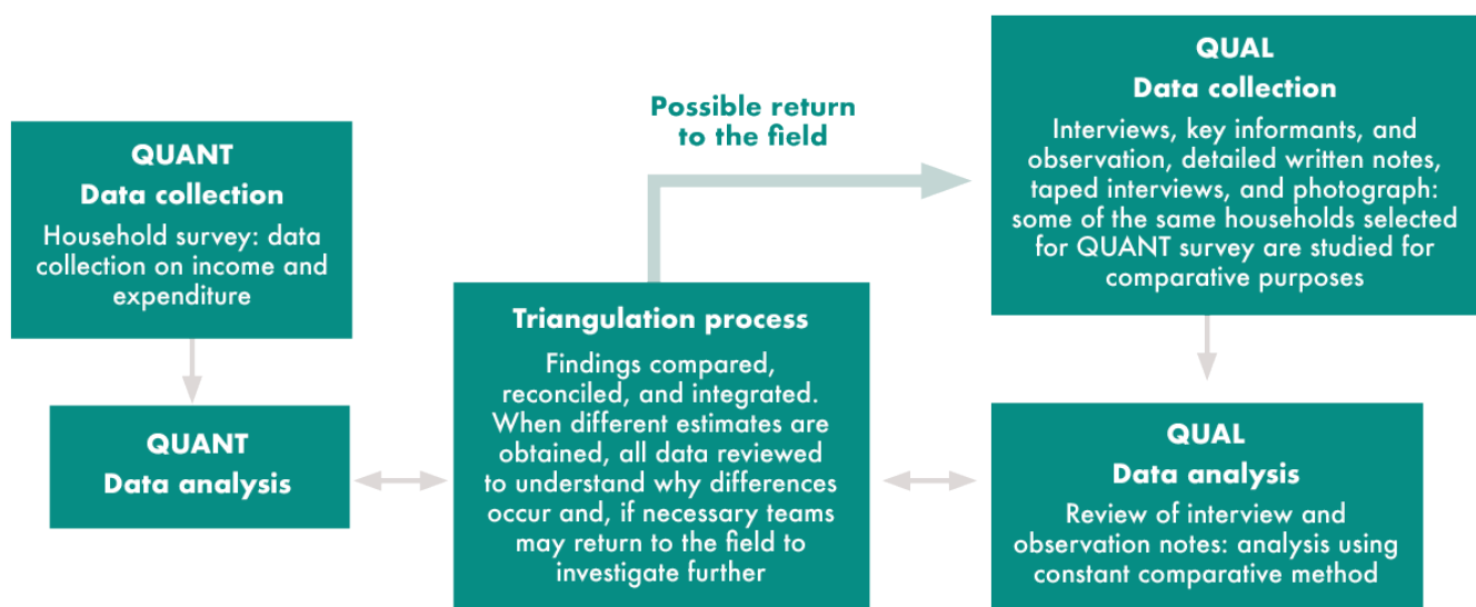
Figure 12. Triangulation framework
