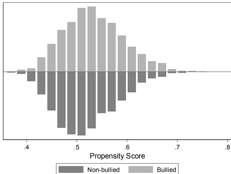
Fig. 1. Propensity score distributions by bully
