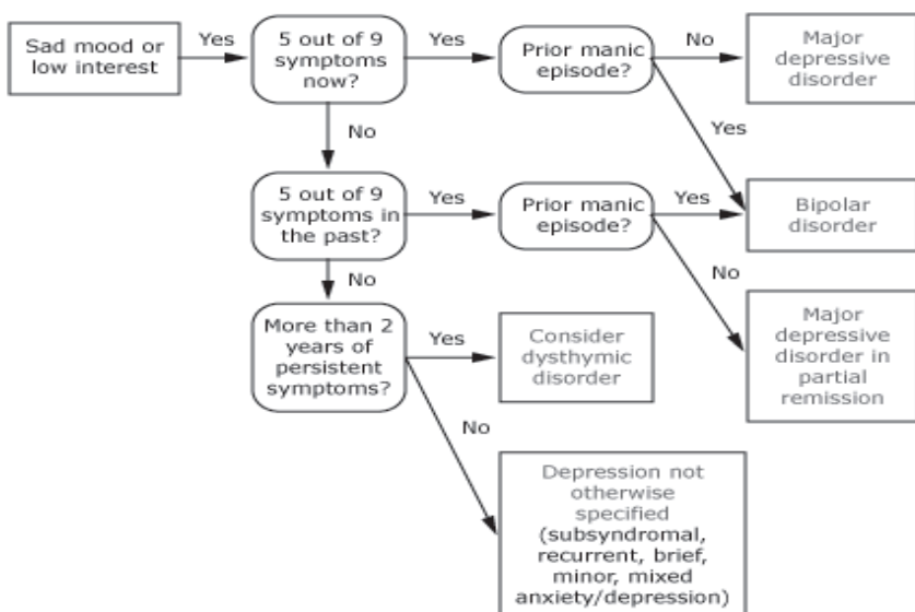
Figure 2-Algorithm for depression
