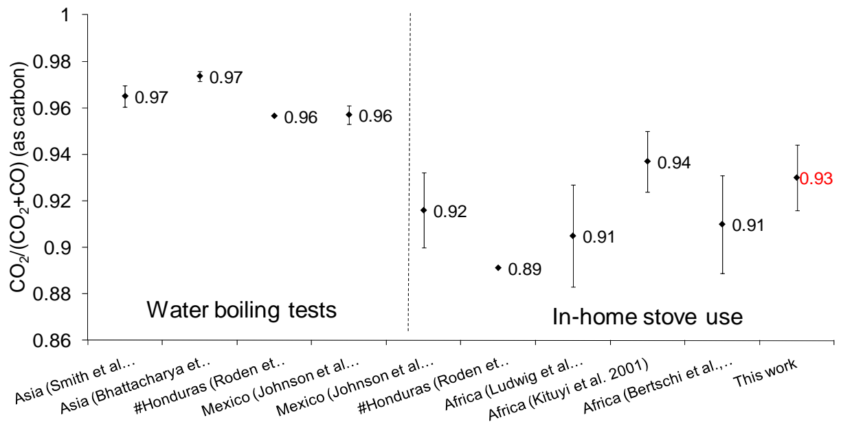
Figure 4. Proxy combustion efficiencies ( \text{CO}_2/[\text{CO}_2+\text{CO}] ) for traditional open-fire stoves. Results from this study are highlighted in red.
