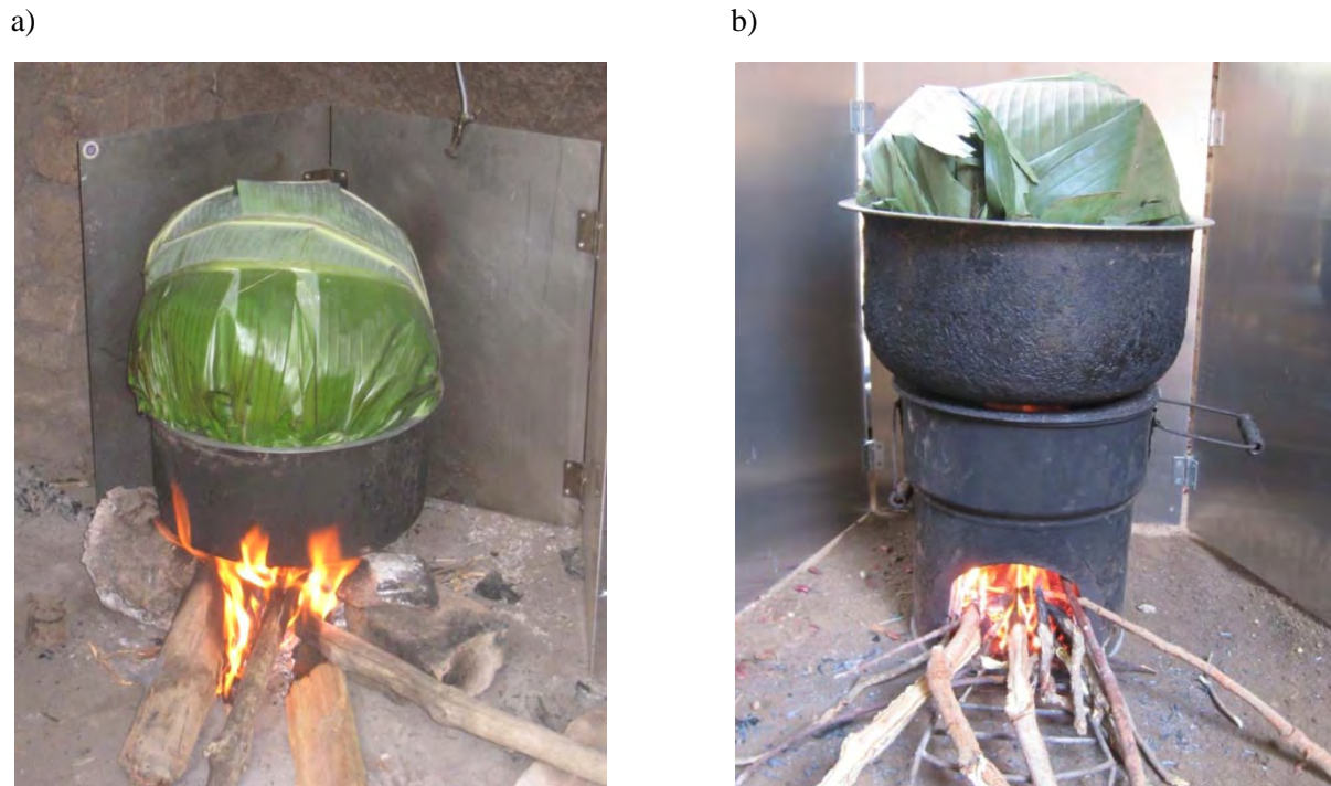
Figure 2. A typical traditional 3-stone fire (a), and the (b) StoveTec rocket stove.
