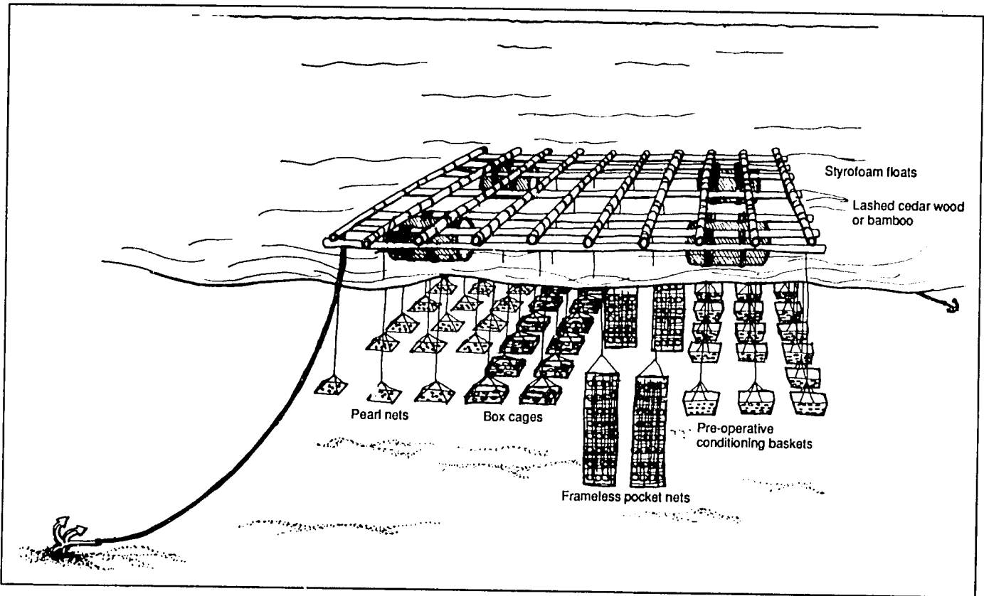
Fig. 7. Typical construction and use of a single raft as used in the pearl culture industry.
