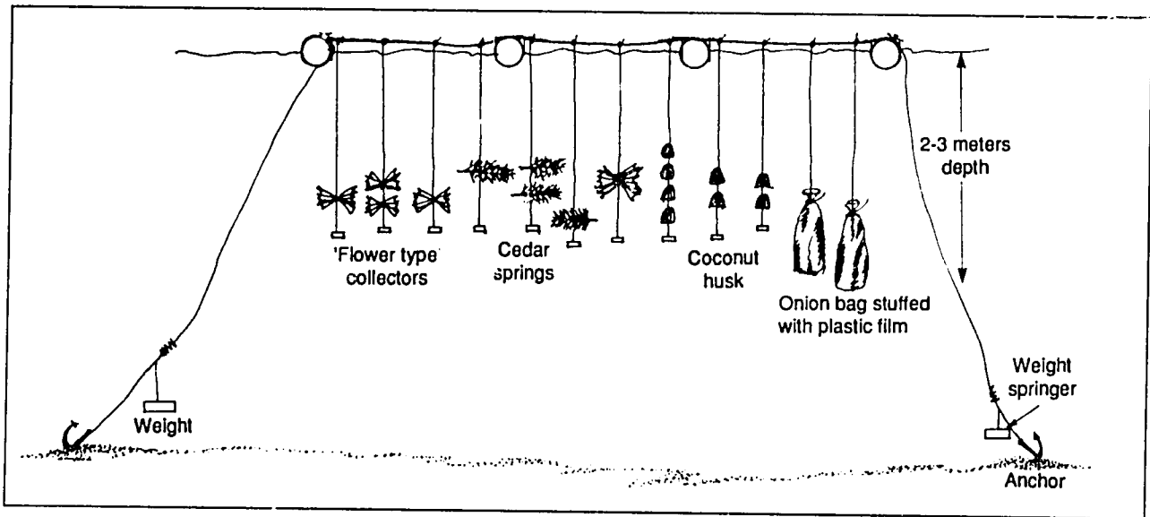
Fig. 5. Diagram of part of a longline showing some materials that may be used for Pinctada spat collection.
