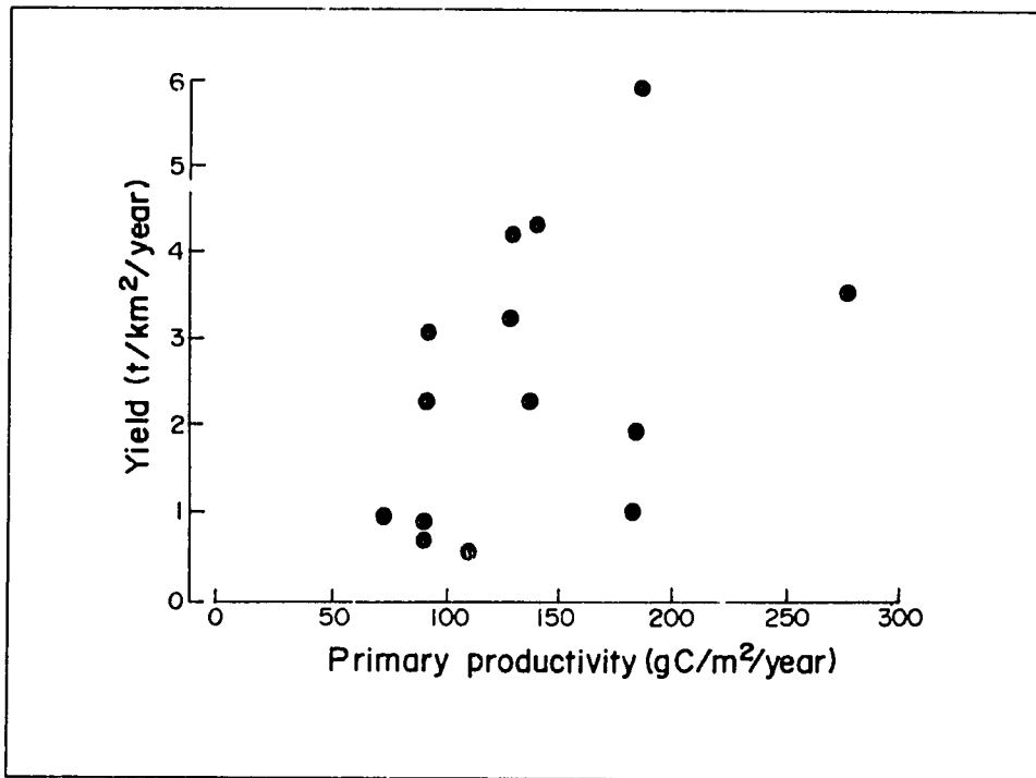
Fig. 9. Maximum sustainable yield and primary productivity of continental shelf pelagic fisheries, based on Table 13. (Source: Marten and Polovina 1982)
