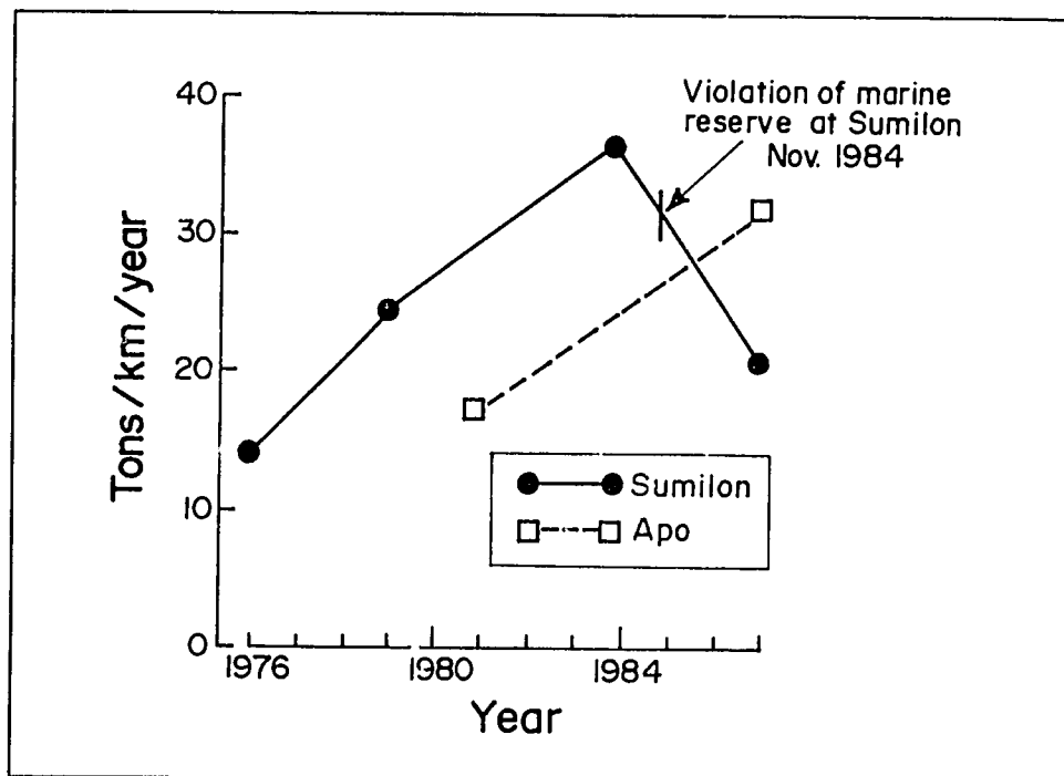
Fig. 7. Change in fish yield reported for Sumilon and Apo Islands, reflecting the effects of different management schemes. (Source: White and Savina 1987)
