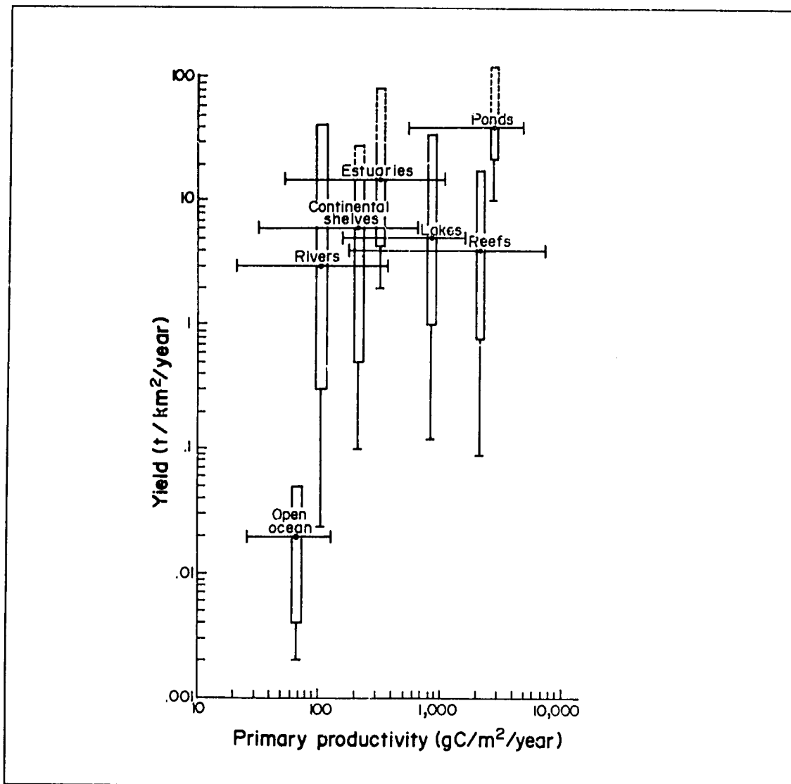
Fig. 10. Ranges of fish yields and primary productivities in various tropical ecosystems. Dots at the intersection of ranges represent modal values. Solid portions of the bars represent the range of maximum sustainable yields. Dashed projections at the top of the ranges for estuaries and ponds represent elevated yields from aquaculture with fertilization (but not supplemental feeding). The dashed projection for continental shelves represents higher yields which occur in areas of upwelling. (Source: Marten and Polovina 1982).
