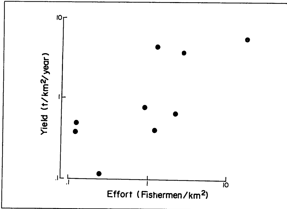
Fig. 6. Fish yields vs fishing effort in coral reefs. (Source: Marten and Polovina 1982)
