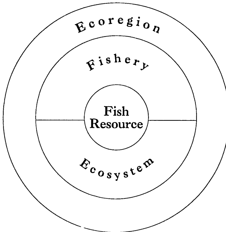
Fig. 3.1. Schematic representation of the nested hierarchies of issues in coastal systems research. The strategy proposed here involves three interconnected "Thrusts", devoted to (1) the FISH RESOURCE and the ECOSYSTEM; (2) the FISHERY; and (3) the ECOREGION.
