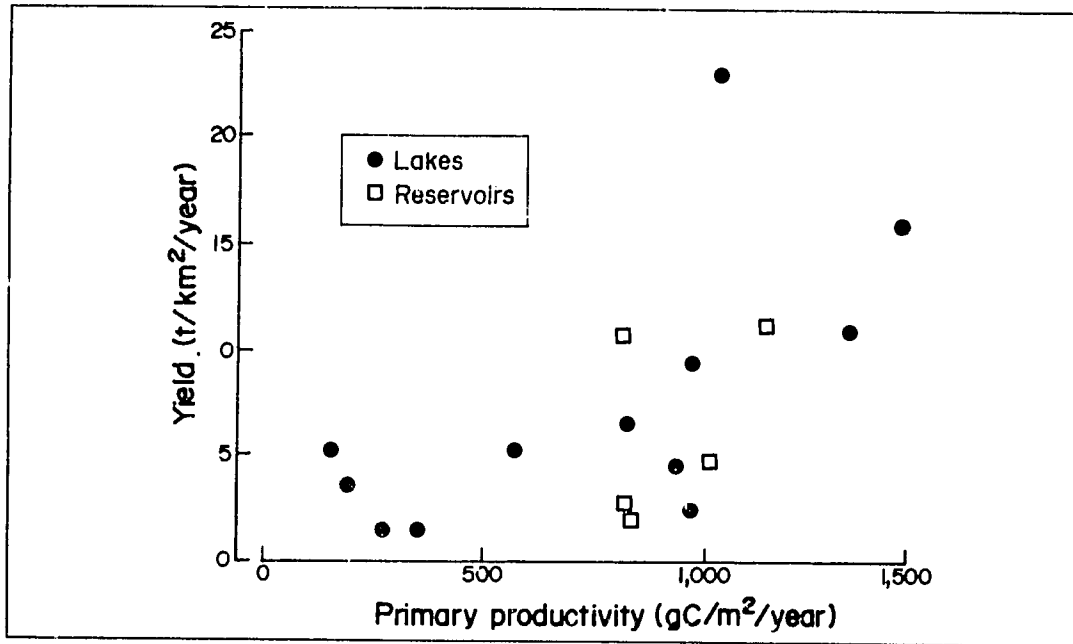
Fig. 2. Fish yields and primary productivity in tropical lakes and reservoirs. (Source: Marten and Polovina 1982)
