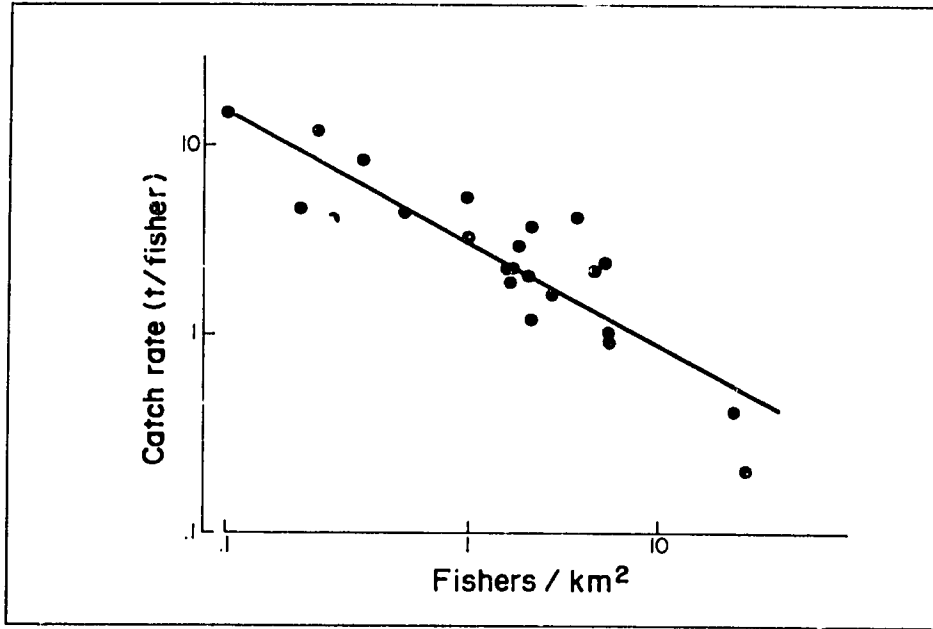
Fig. 4 Catch per unit effort as a function of effort for 17 rivers; CPUE = 2.92 * (Fisheries/km^2)^{-0.4} . (Source: Welcomme 1985).
