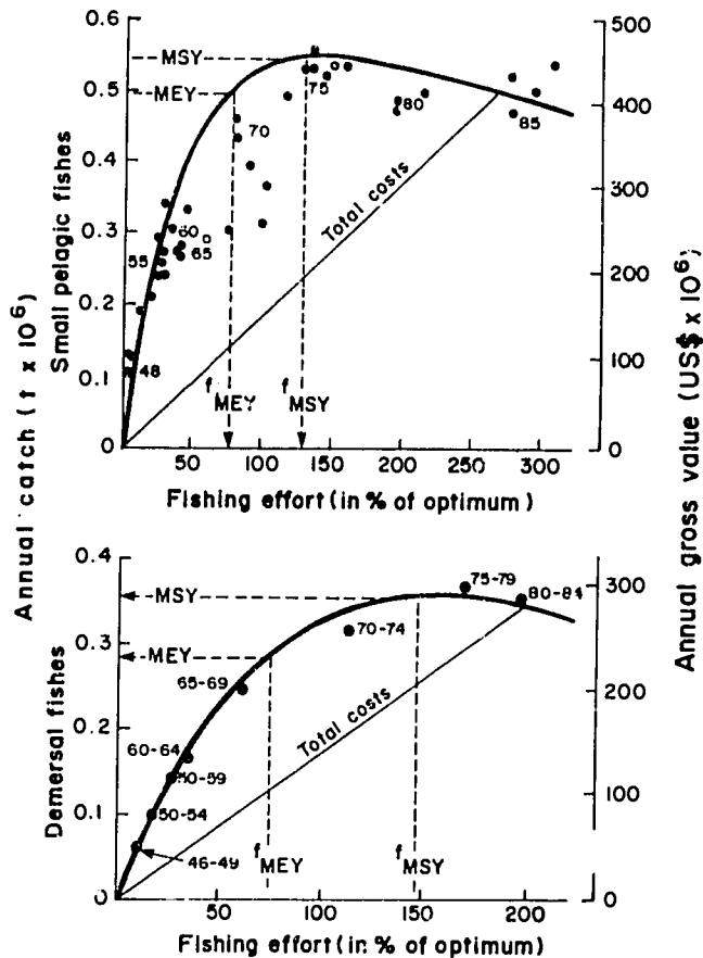
Surplus production models of the Philippine pelagic and demersal fisheries; both models provide rough estimates of total fishing costs and economic rent through the crude assumption of equilibrium in the early 1980s. Fishing effort is expressed in %, relative to the effort required to extract a catch intermediate between maximum economic and maximum sustainable yield (MEY and MSY) (these terms are defined in Illustration 2). Note need for drastic reduction of effort for both resource types.
