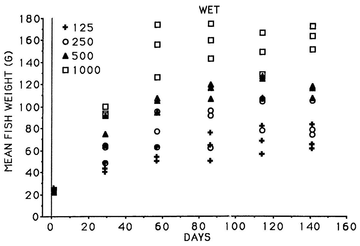
Figure 1. Mean weight gain of Oreochromis niloticus during Cycle III, dry and wet seasons at Gualaca, Panama. Chicken litter inputs (treatments) were 125, 250, 500, and 1000 kg/ha/wk, total solids.
