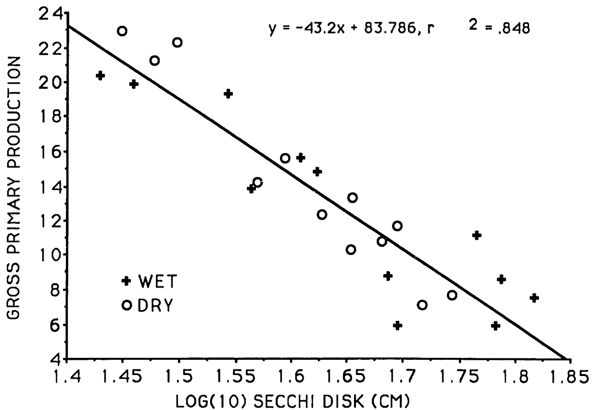
Figure 15. Regression of mean Secchi disk visibility on chlorophyll a (log transformed), and gross primary production (mg O 2 /l/d) on Secchi disk visibility (log transformed) during Cycle III, dry and wet seasons combined, at Gualaca, Panama.
