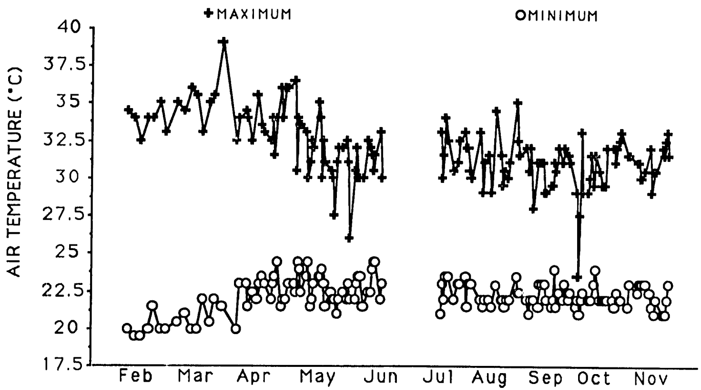
Figure 11. Solar radiation (Einsteins/m 2 /d), and maximum and minimum air temperatures during the dry (January to June) and wet (July to December) seasons of Cycle III at Gualaca, Panama.
