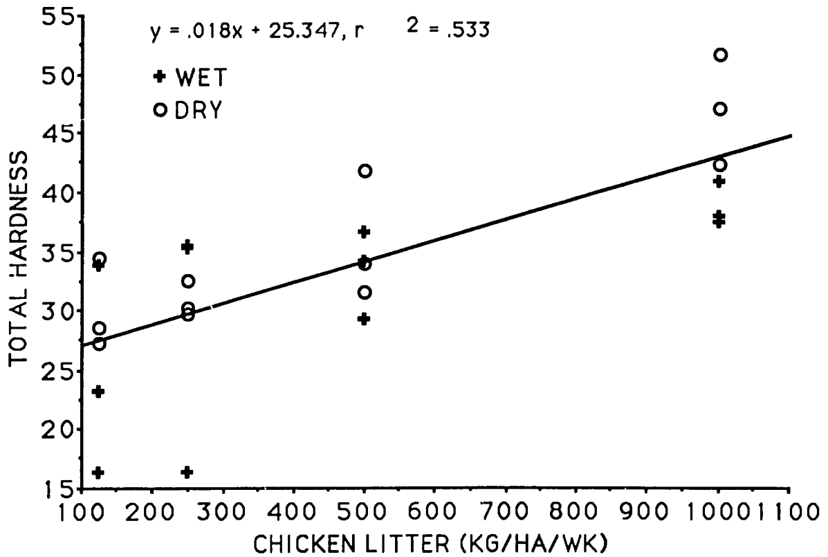
Figure 6. Regression of mean total alkalinity (mg CaCO 3 /l) and total hardness (mg CaCO 3 /l) on chicken litter application during Cycle III, dry and wet seasons combined, at Gualaca, Panama.
