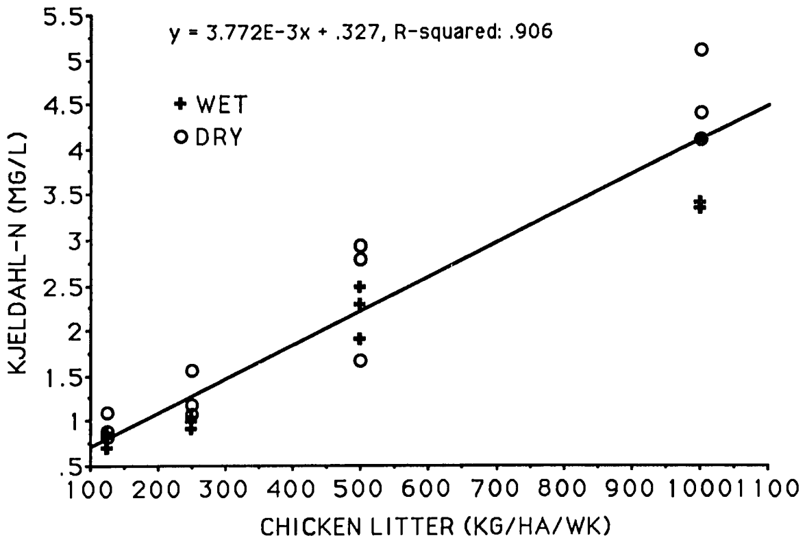
Figure 5. Regression of mean total ammonia nitrogen and Kjeldahl nitrogen on chicken litter application during Cycle III, dry and wet seasons combined, at Gualaca, Panama.
