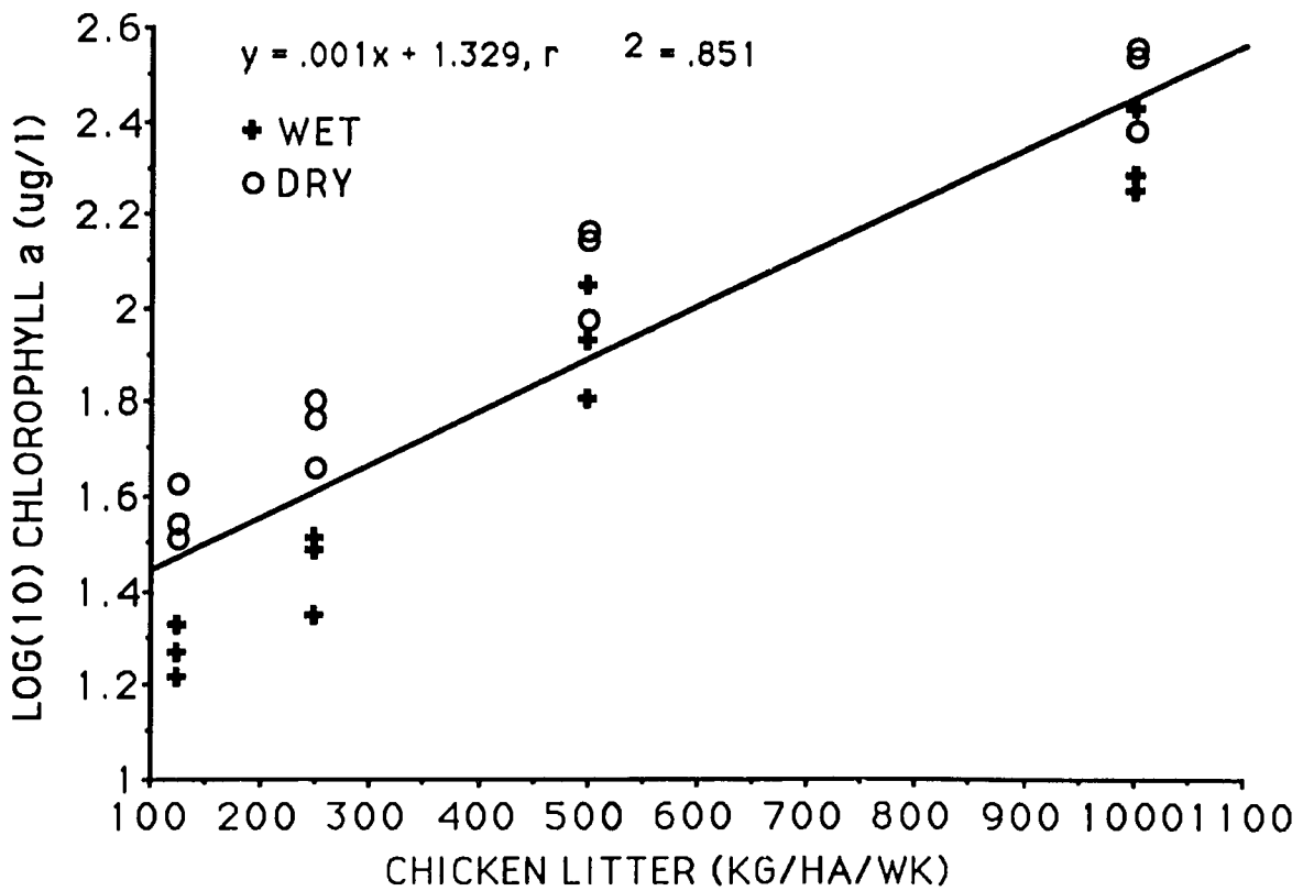
Figure 8. Regression of mean Secchi disk visibility (log transformed), and chlorophyll a (log transformed) on chicken litter application during Cycle III, dry and wet seasons combined, at Gualaca, Panama.
