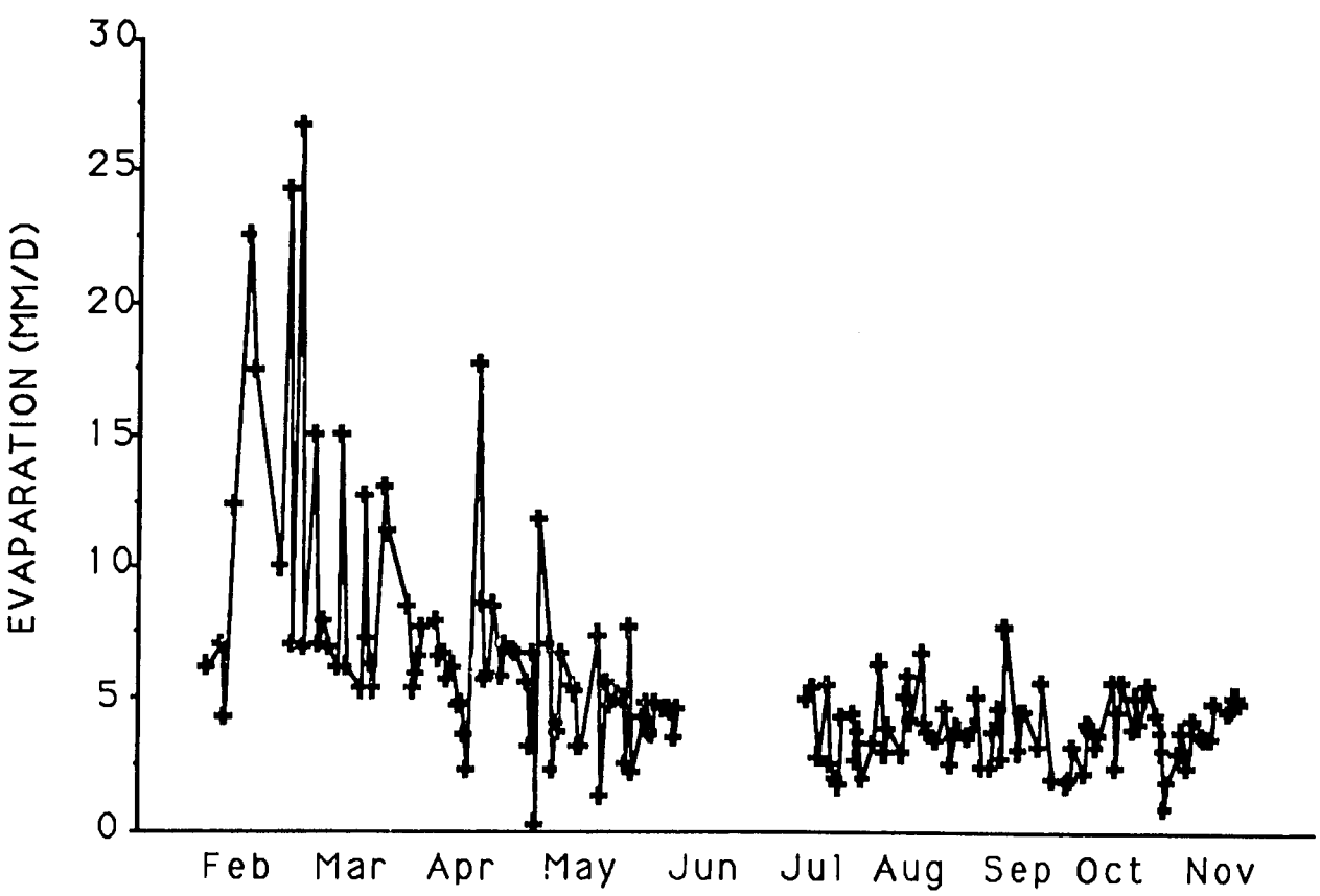
Figure 10. Rainfall and pond evaporation (pan evaporation X 0.83) during the dry (January to June) and wet (July to December) seasons of Cycle III at Gualaca, Panama.
