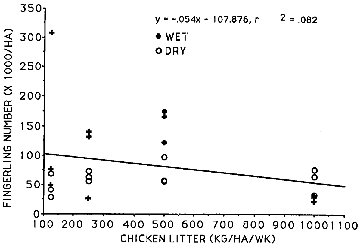
Figure 2. Regression of fingerling production and number of fingerlings on chicken litter application during Cycle III, dry and wet seasons combined, at Gualaca, Panama.
