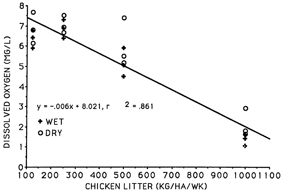
Figure 7. Regression of mean early morning dissolved oxygen concentration on chicken litter application during Cycle III, dry and wet seasons combined, at Gualaca, Panama.
