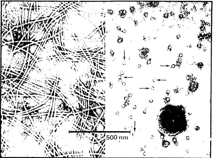
Characteristic virus particles as seen with the electron microscope include filaments (PVY), and isometric (PLRV) particles (1 nm = 0.000 001 mm).
