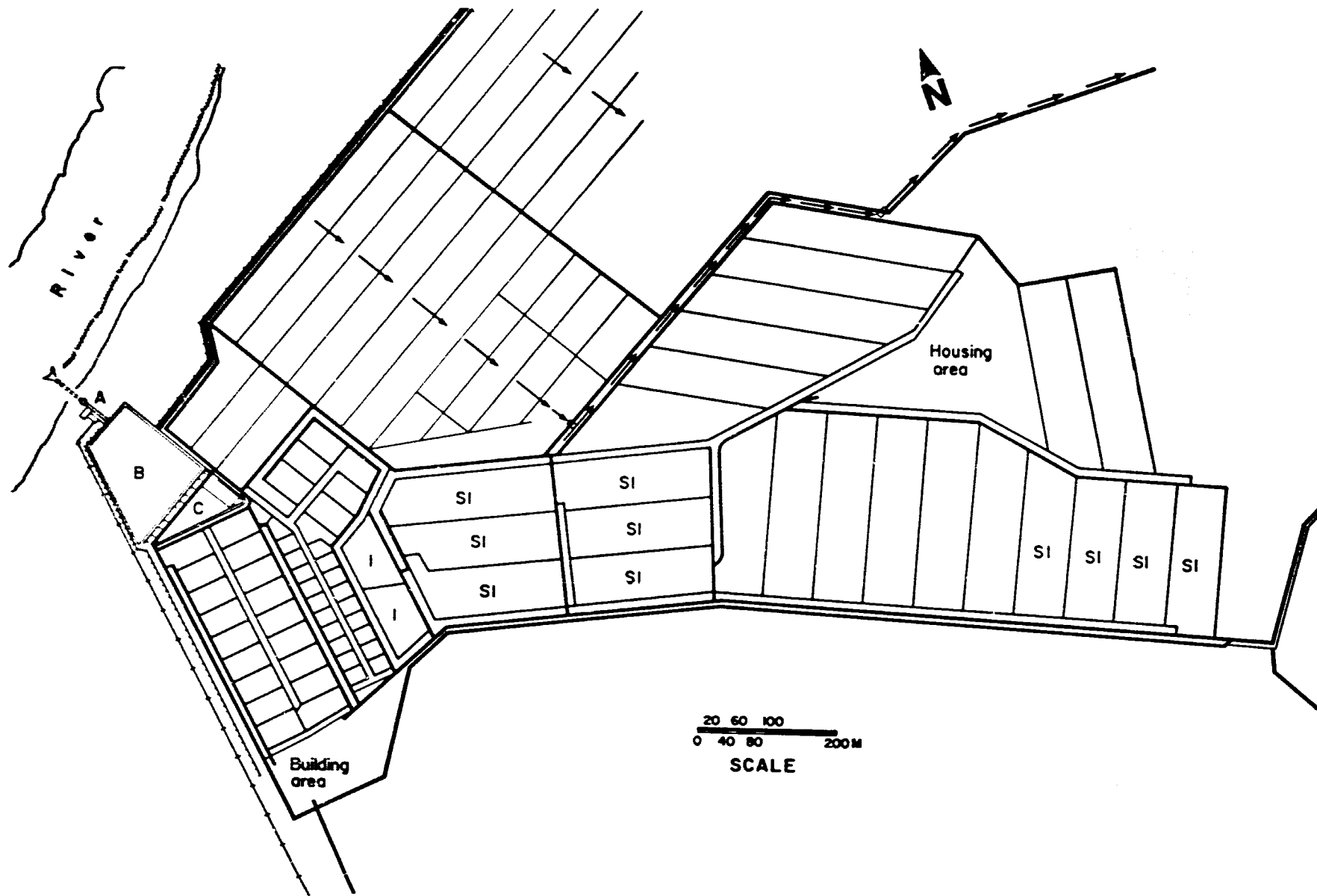
Figure 1. Design of the proposed Tha Ngone pilot fish farm. Smallest ponds are nursery ponds. Above and left are spawners and rearing ponds. I, intensive ponds, SI, semi-intensive. Remainder of ponds are for extensive farming. The fish farm is part of a large agricultural complex. Arrows show flow of irrigation water through fields. A, irrigation pumping system. B, irrigation regulating pond. C, fish farm regulating pond.
