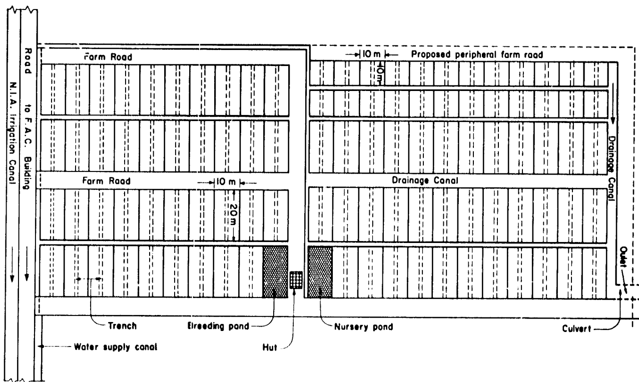
Figure 2. Layout of rice-fish culture area at the Freshwater Aquaculture Center, Central Luzon State University. Scale 1:1,000.
