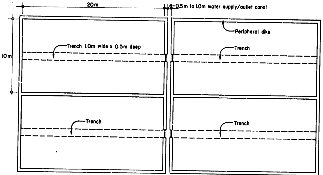
Figure 4. Location of trench for a 10m x 20m paddy. Scale 1:200.
