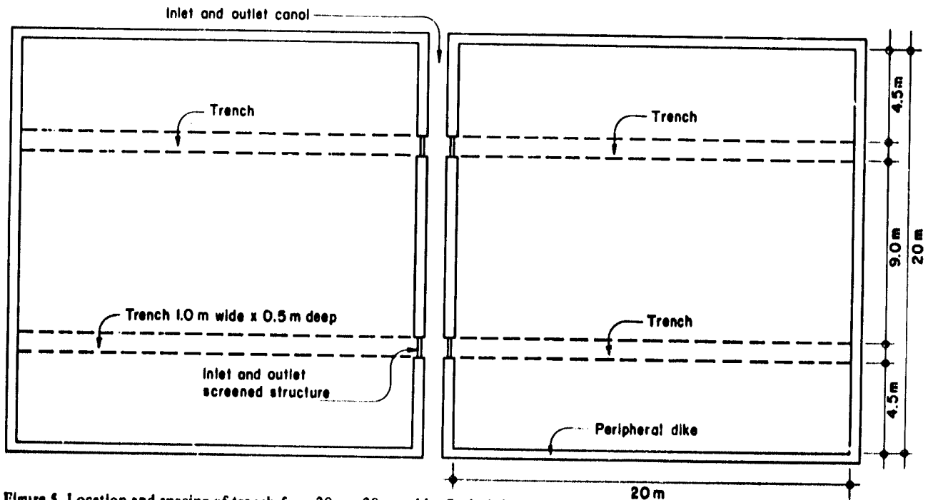
Figure 5. Location and spacing of trench for a 20m x 20m paddy. Scale 1:200.
