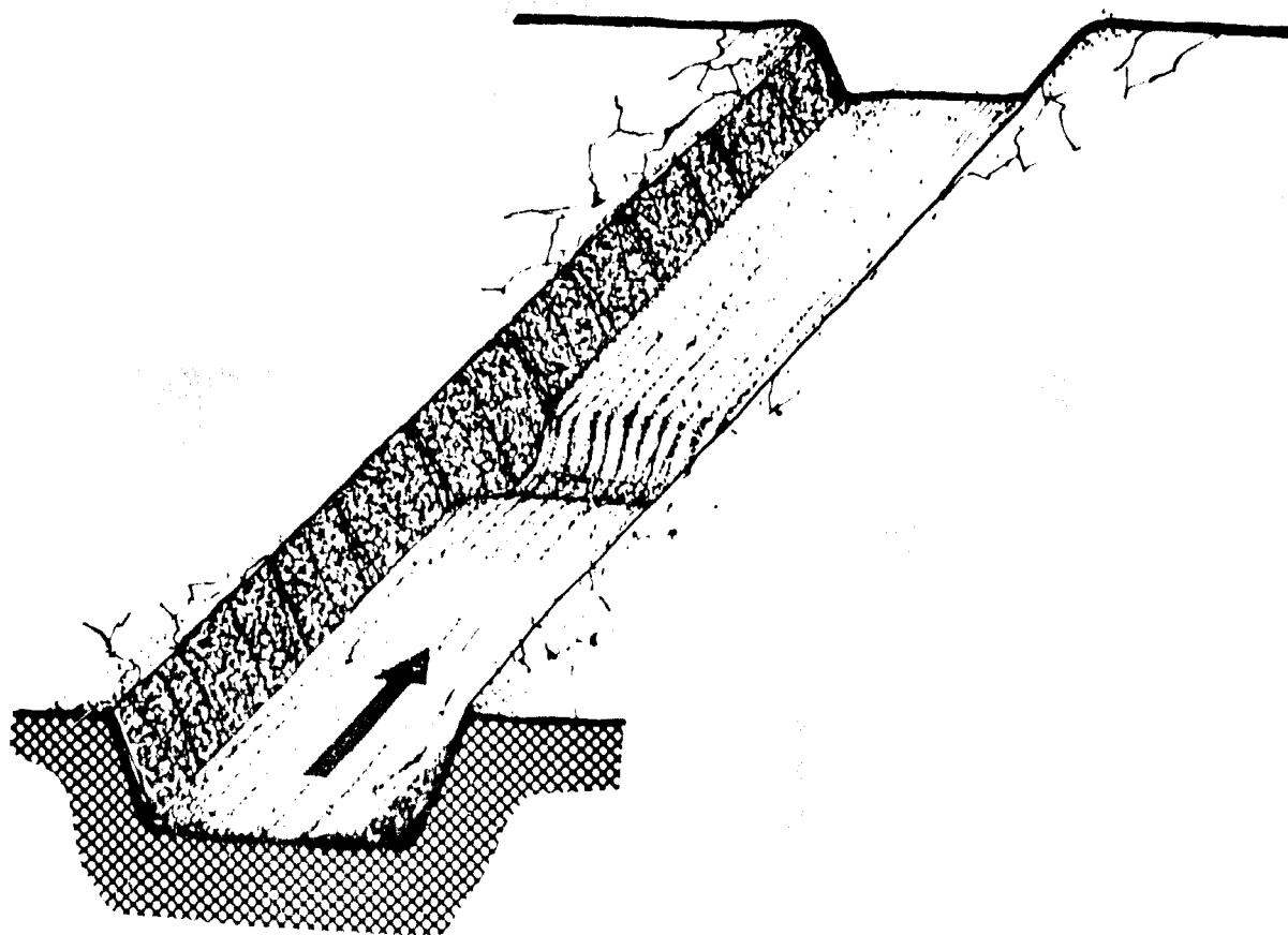
Figure 8. Cross sectional view of a deepened trench to serve as a fish refuge during water lowering in rice-fish culture: the arrow indicates direction of flow from inflow to drain.
