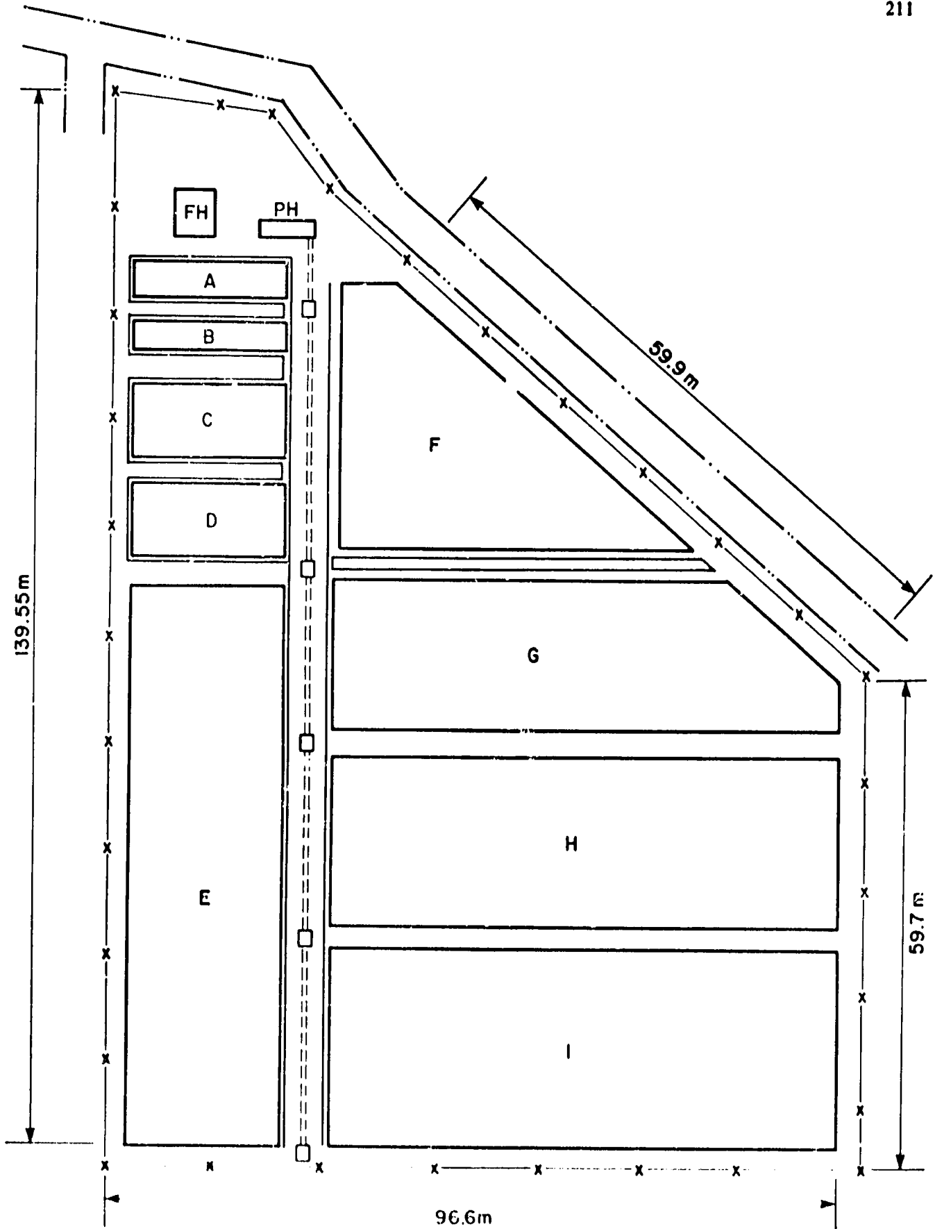
Figure 1. Layout of the Central Luzon State University model farm. A & B, nursery ponds. C & D, breeding ponds. E, F, rice fish paddies. FH, model farm house. PH, pump house. Scale 1:200
