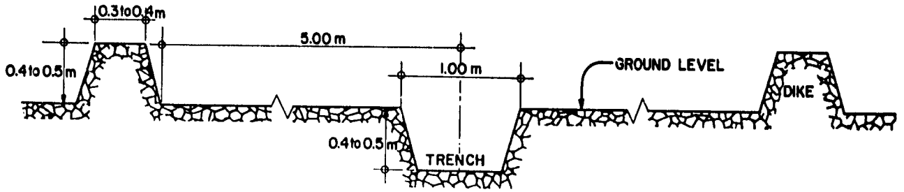
Figure 3. Cross section of paddy, dike and trench (not drawn to scale).
