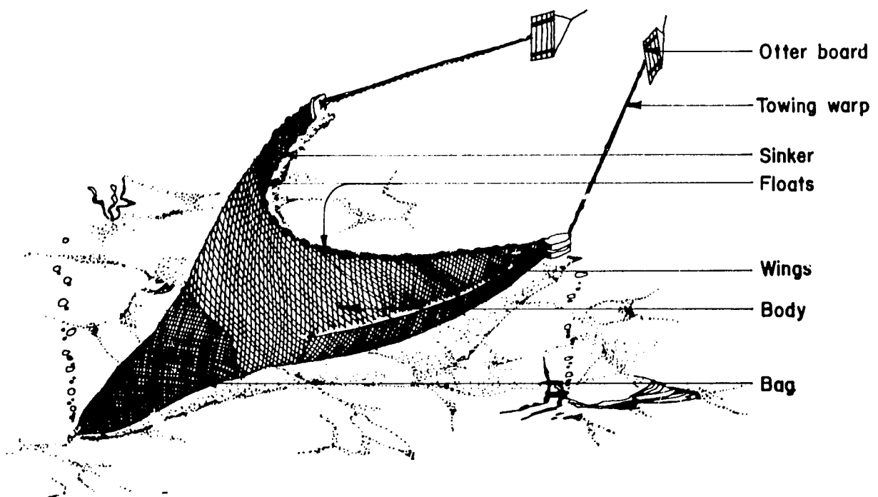
Fig. 17. An ordinary otter trawl. Baby trawls use this and other trawl gear.
