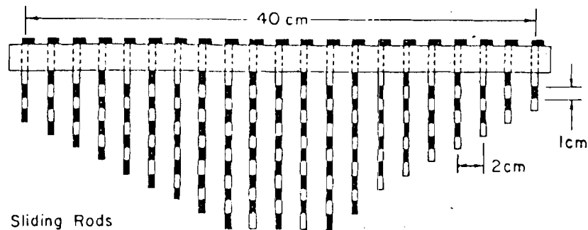
Figure 9. Furrow profilometer.
