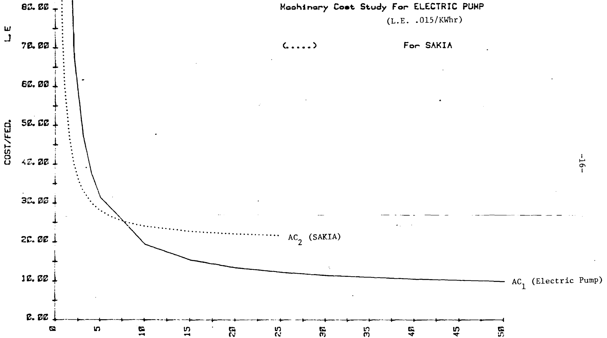
Figure 3 Comparisons of Pumping Costs When Current Charge For Electricity Used
