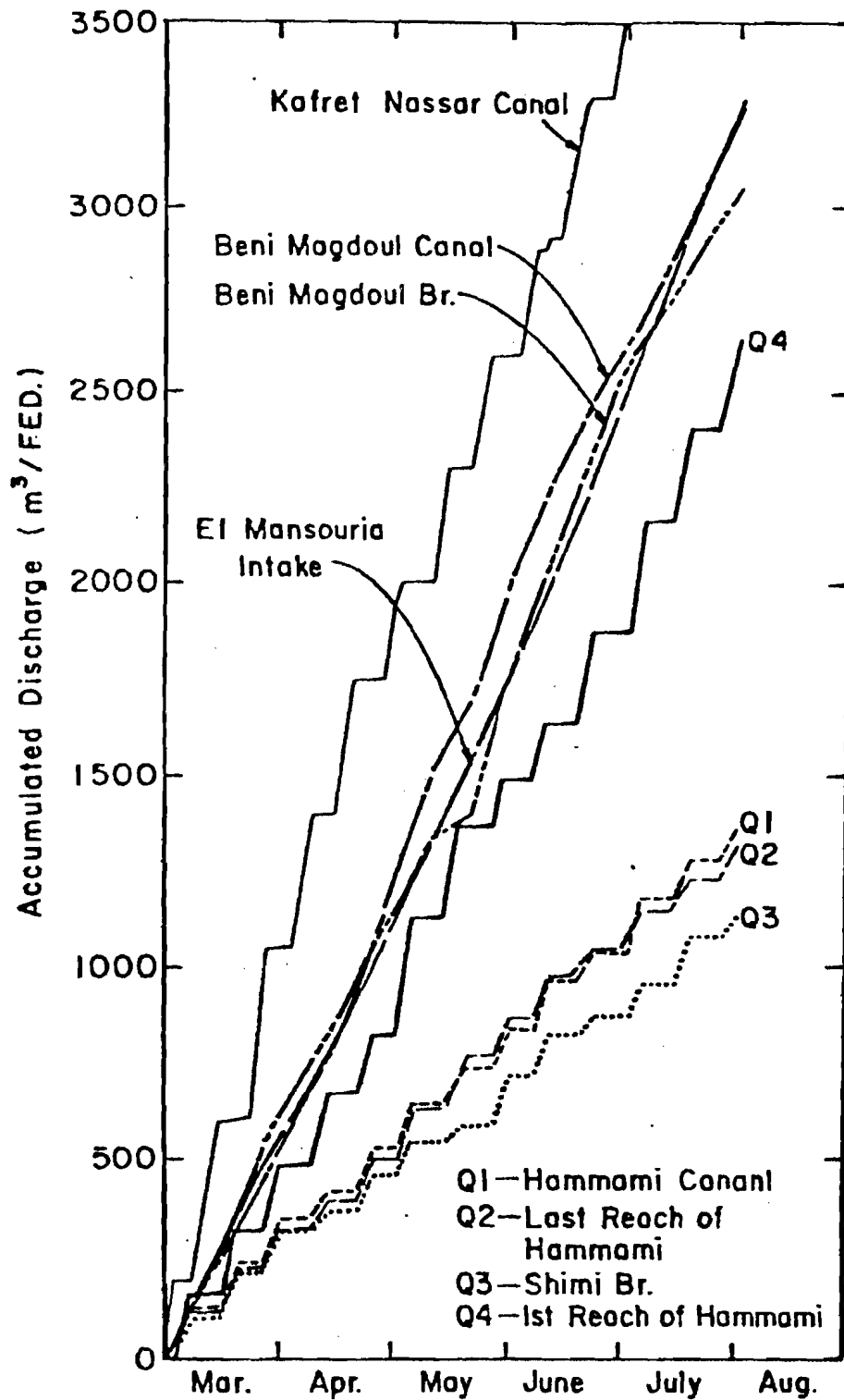
Figure (2) Accumulated discharges as measured at the upstream head gates for the Mansouria Canal and three of its laterals as a function of time for 1978.
