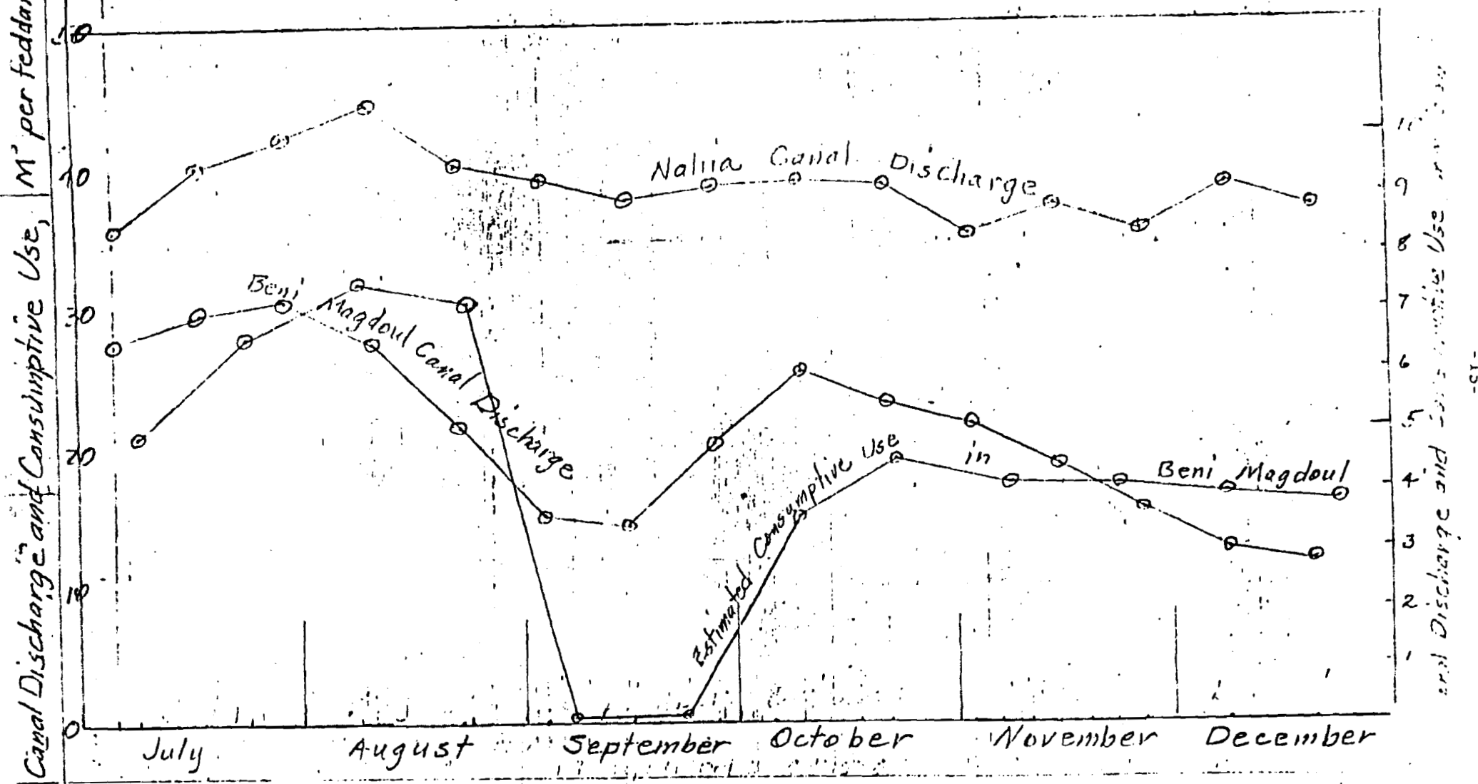
Figure 1. Comparisons among the discharge in the Beni Magdoul Canal, the Nahia Canal, and the estimated consumptive use in Beni Magdoul during the last half of 1979
