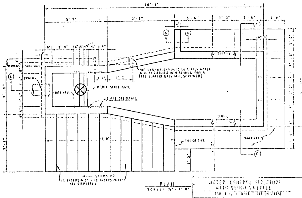
Fig. 5. Construction diagram of a typical water control structure and catch basin (seining kettle). Located in the deep end of the pond, this structure facilitates removal of the small fish with the minimum amount of stress.
