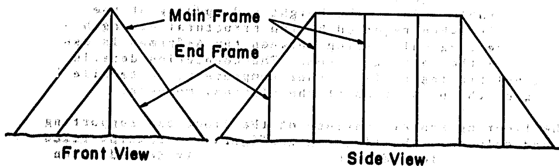
Figure 3 A-Frame Elevation
