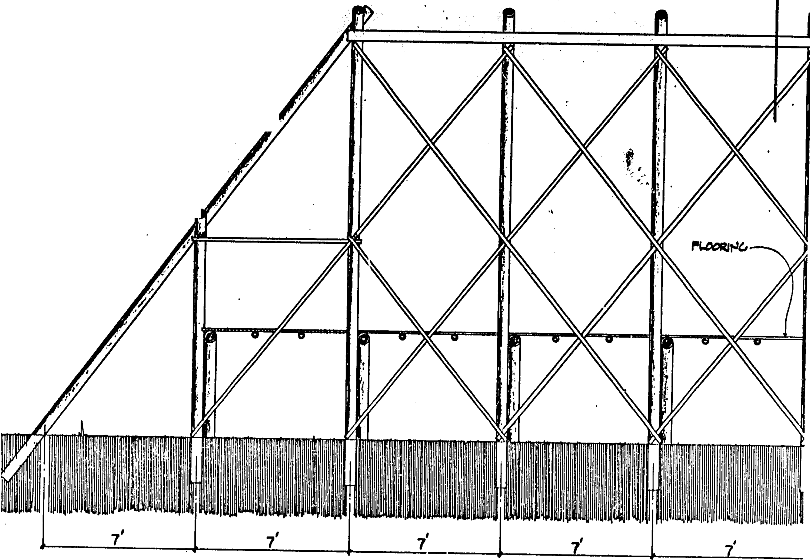
ONE LIVING UNIT STRUCTURAL ELEV.
