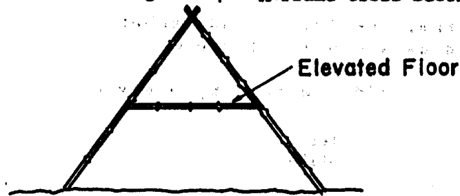
Figure 4 A-Frame Cross Section
