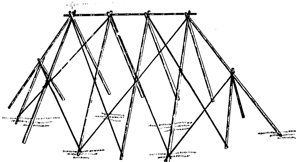
CROSS BRACING BETWEEN FRAMES 90° INTERSECTIONS
