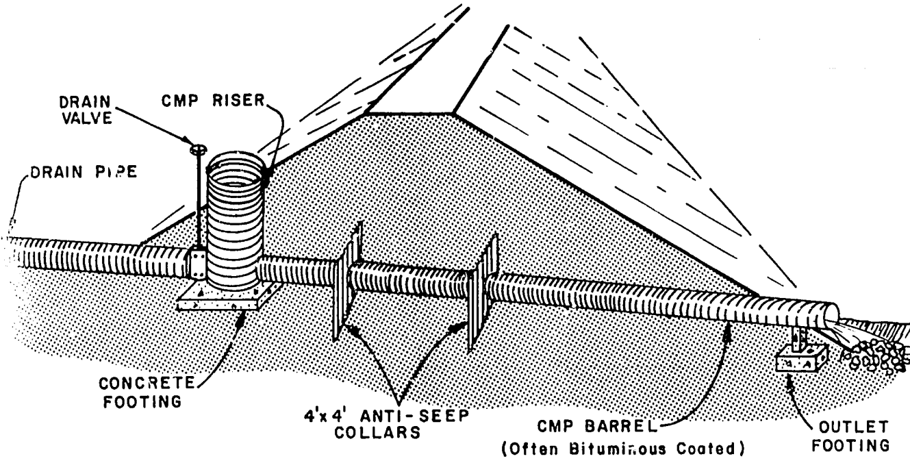
FIGURE 18 - CORRUGATED METAL PIPE OUTLET WORKS
