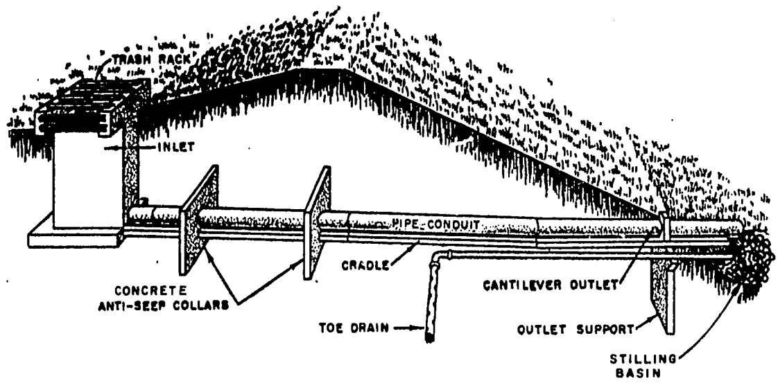
FIGURE 14 - REINFORCED CONCRETE INLET AND PIPE (U. S. Soil Conservation Service, 1969)
