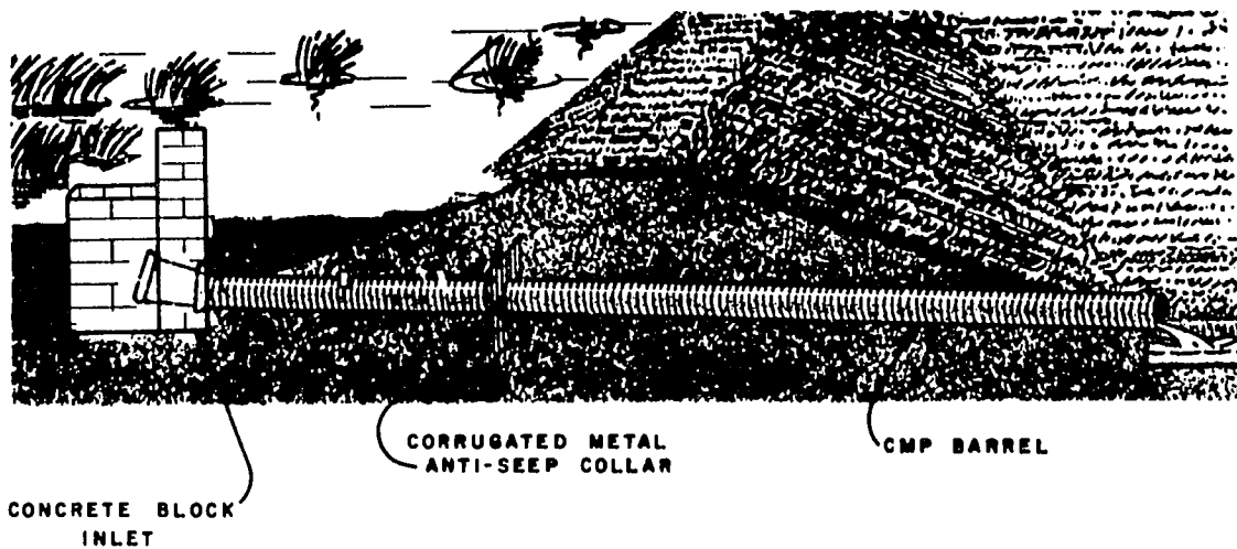
FIGURE 15 - CONCRETE BLOCK INLET WITH CMP BARREL
