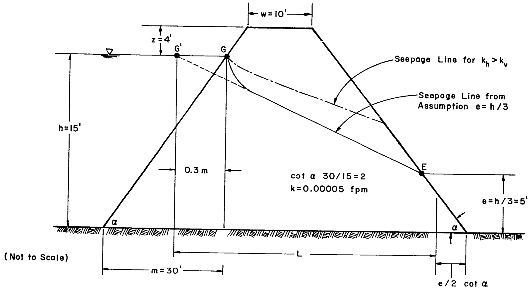
FIGURE A4 - APPROXIMATE METHOD OF SEEPAGE DETERMINATION
