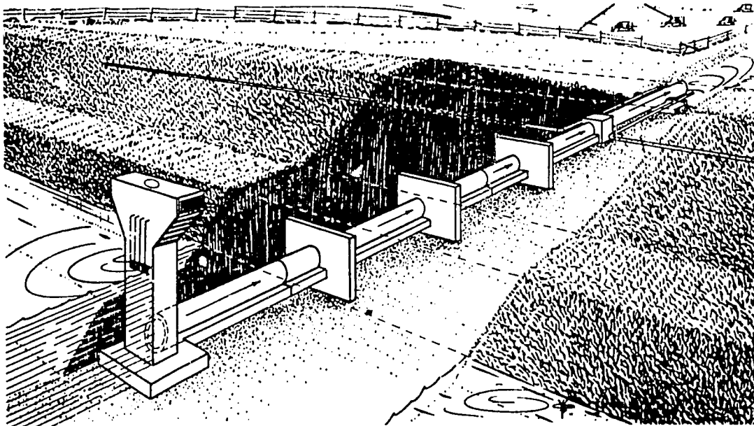
FIGURE 13 - OUTLET WITH MULTI-STAGE INLET ( U.S. Soil Conservation Service , 1969 )
