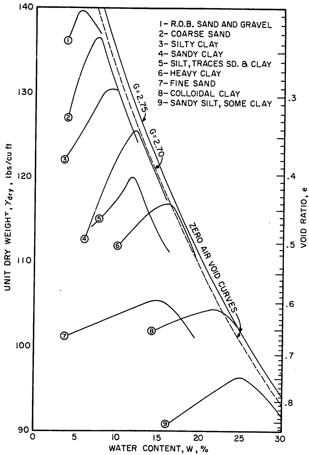
FIGURE B5 - TYPICAL PROCTOR TEST CURVES (B.K. Hough, 1969)
