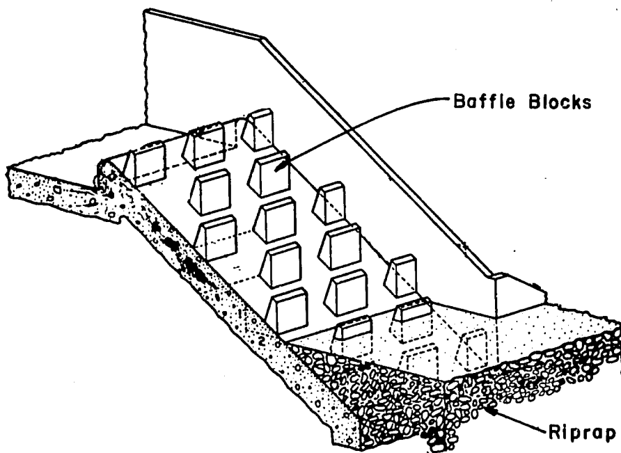
(b) Reinforced Concrete Basin
