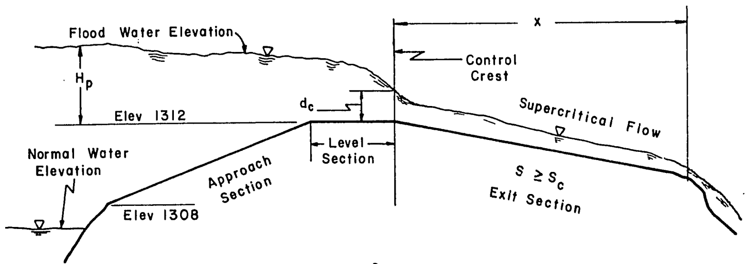
(b) Profile Along \mathcal{C} of Spillway
