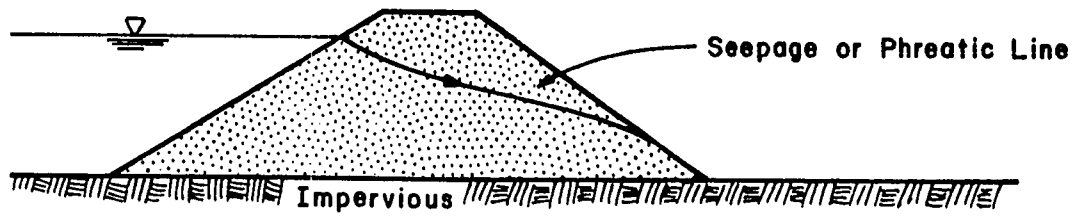
(a) Impervious Foundation without Drainage
