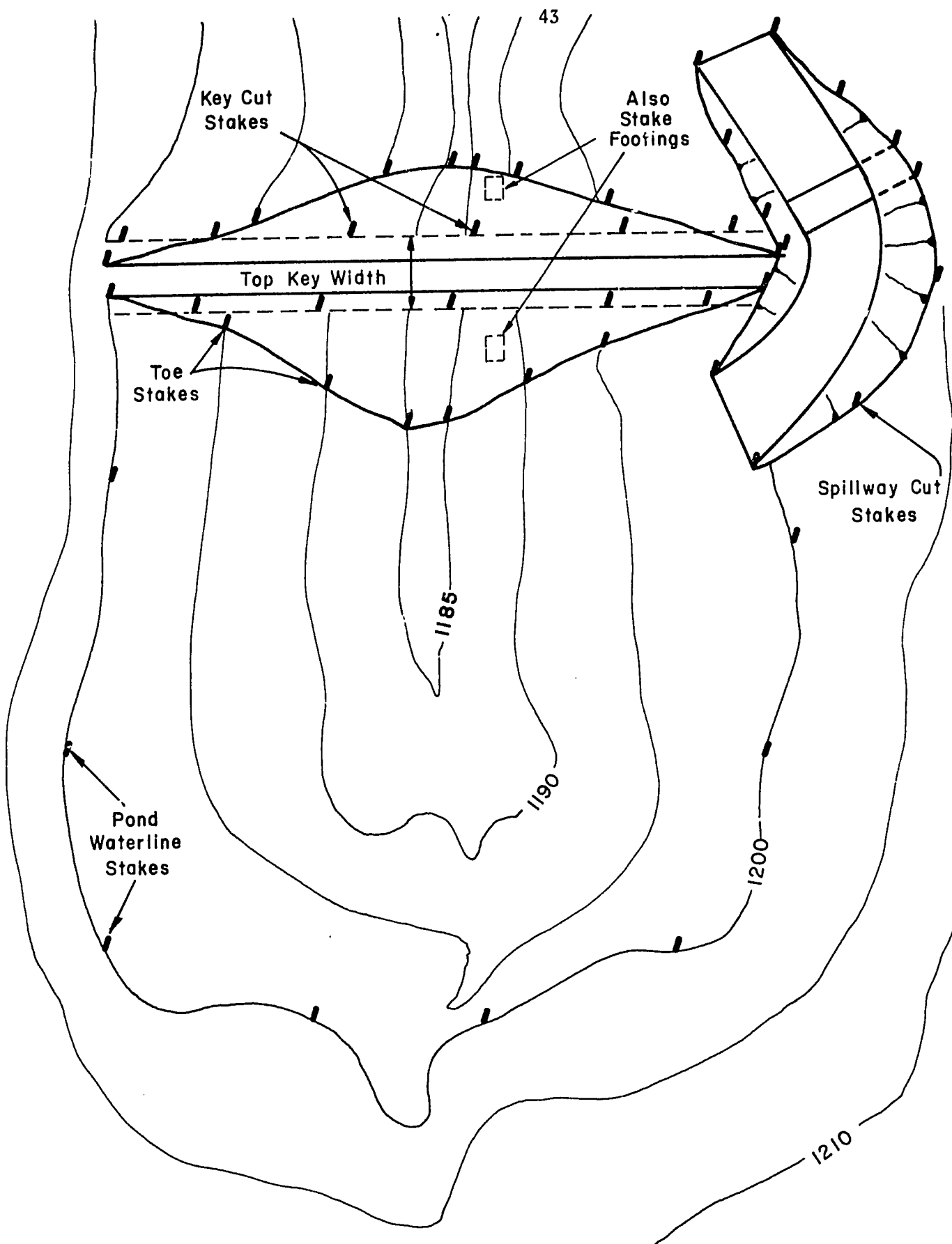
FIGURE 27 - STAKING LAYOUT
