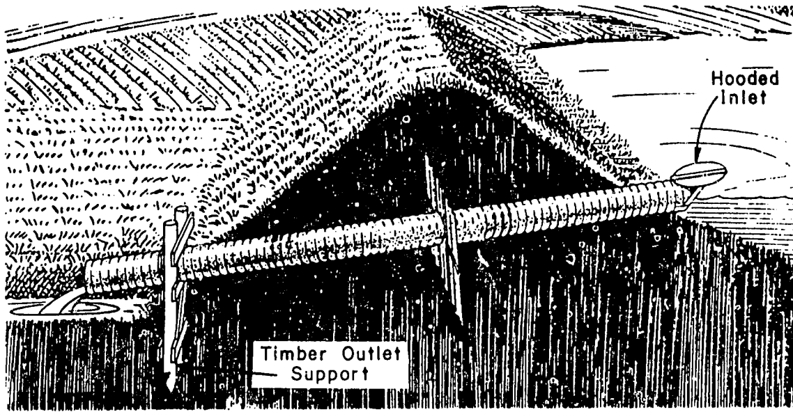
FIGURE 16- HOOD CMP OUTLET (U.S. Soil Conservation Service, 1969)
