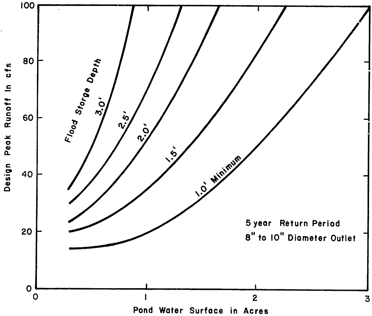
FIGURE 9 - SUGGESTED FLOOD STORAGE DEPTH (Schwab, G.O., et al. Soil and Water Conservation Engineering )
