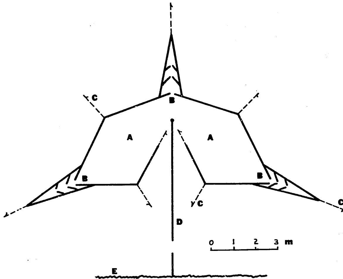
Figure 10. Pound net of three traps used to harvest shrimp from ponds. A. body of net; B. funnel traps; C. anchor lines; D. wing net; and, E. pond dike.
