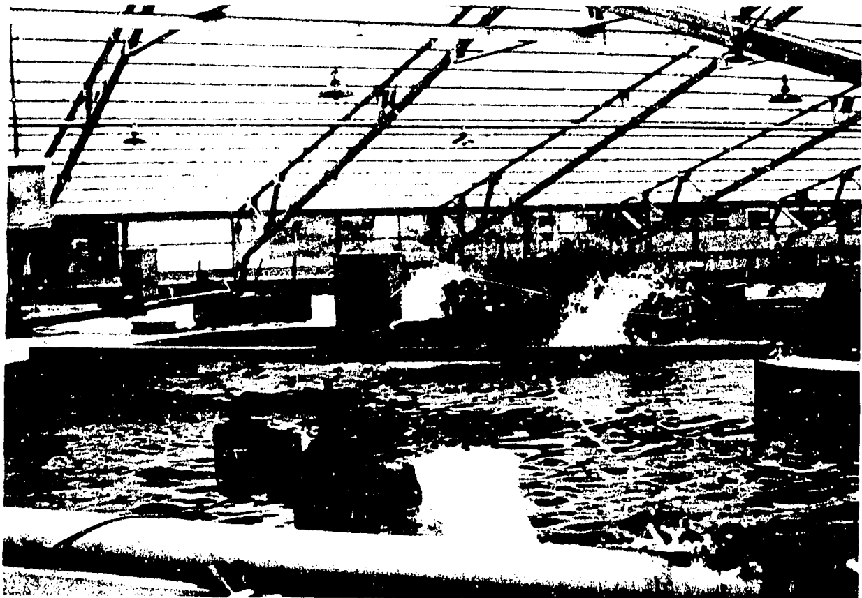
Figure 4. Octagonal concrete raceways for ayu culture within fiberglass building. Note water inlet in foreground and automatic feeder in center.
