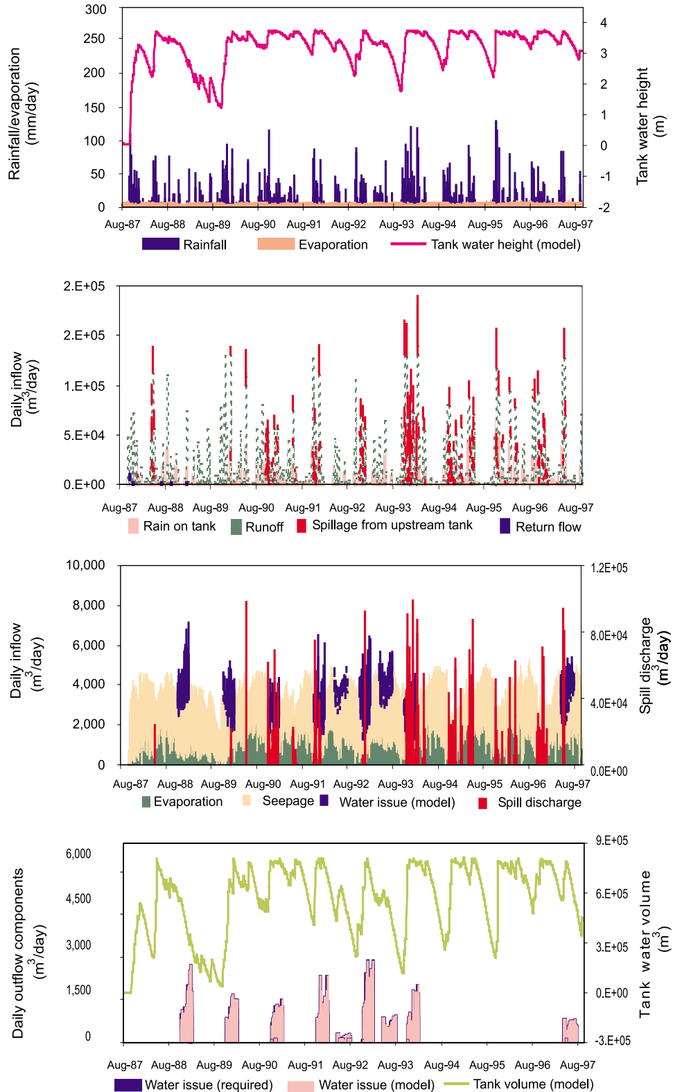
FIGURE 14. Predicted tank water height, volume, and tank water balance components—Alisthana.
