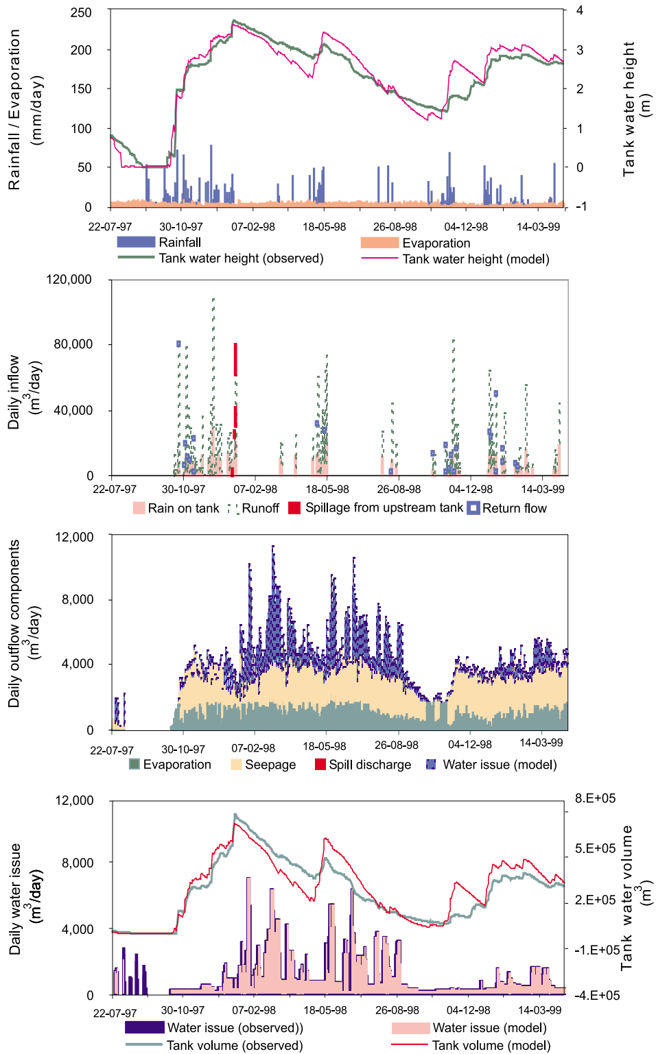
FIGURE 9. Model calibration: Observed and simulated tank water height, volume, and simulated tank water balance components—Alisthana.
