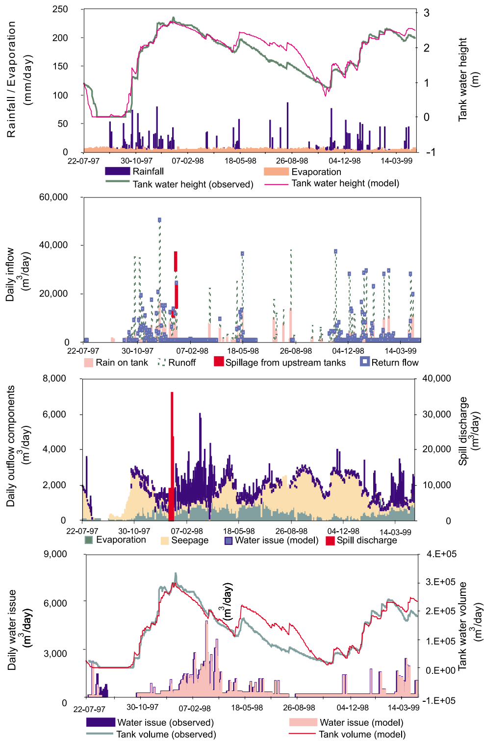
FIGURE 8. Model calibration: Observed and simulated tank water height, volume, and simulated tank water balance components—Meegassagama.
