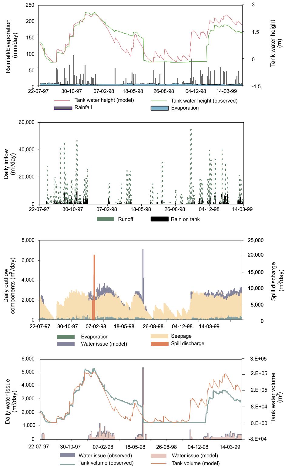
FIGURE 6. Model calibration: Observed and simulated tank water height, volume, and simulated tank water balance components—Vendarankulama.
