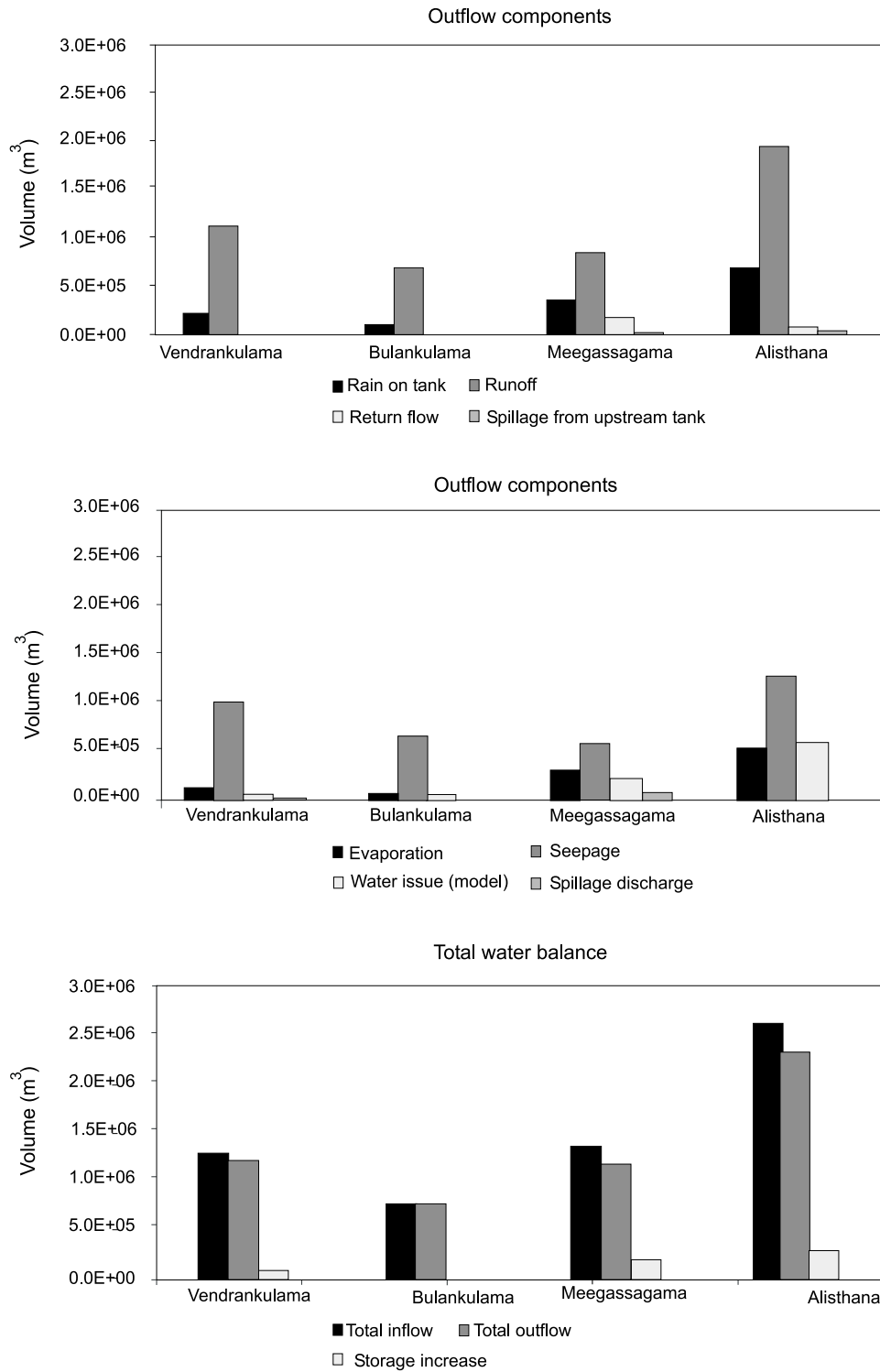
FIGURE 10. Total water balance of the tank cascade system over the calibration period.
