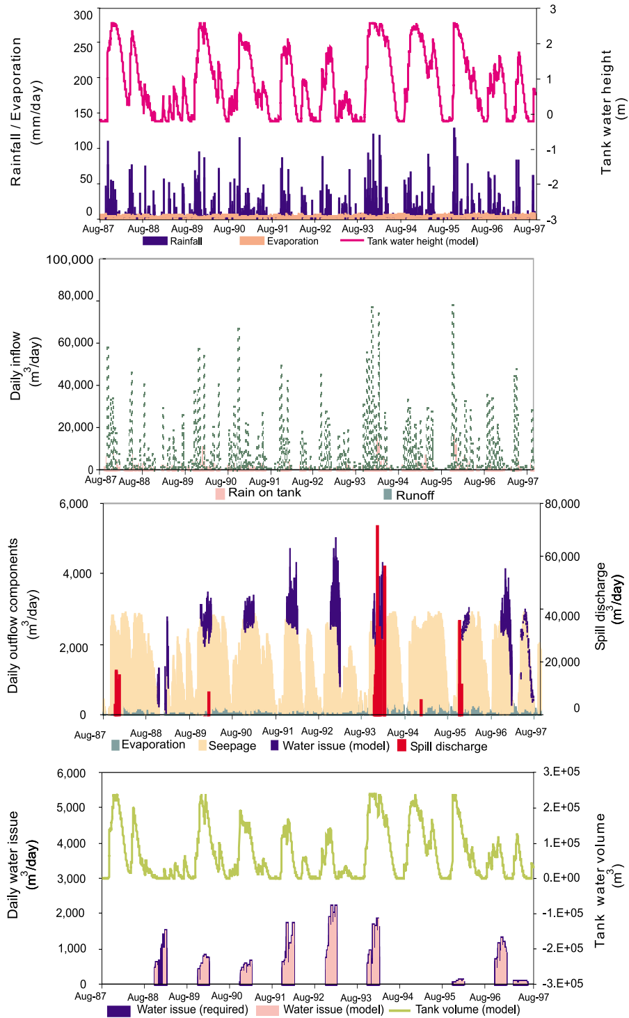
FIGURE 11. Predicted tank water height, volume, and tank water balance components–Vendarankulama.
