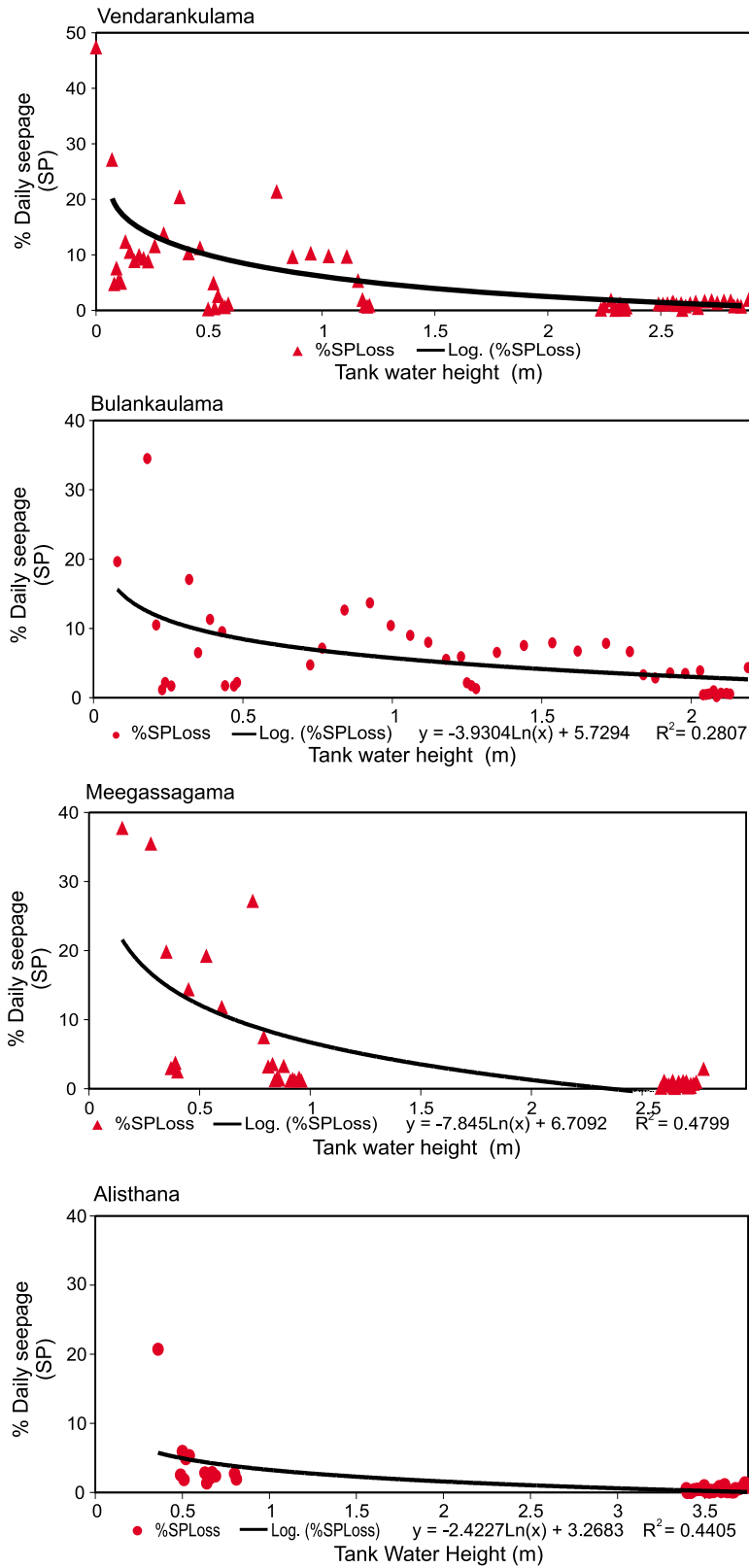
FIGURE A.1. Percent seepage as a function of the tank water height.
