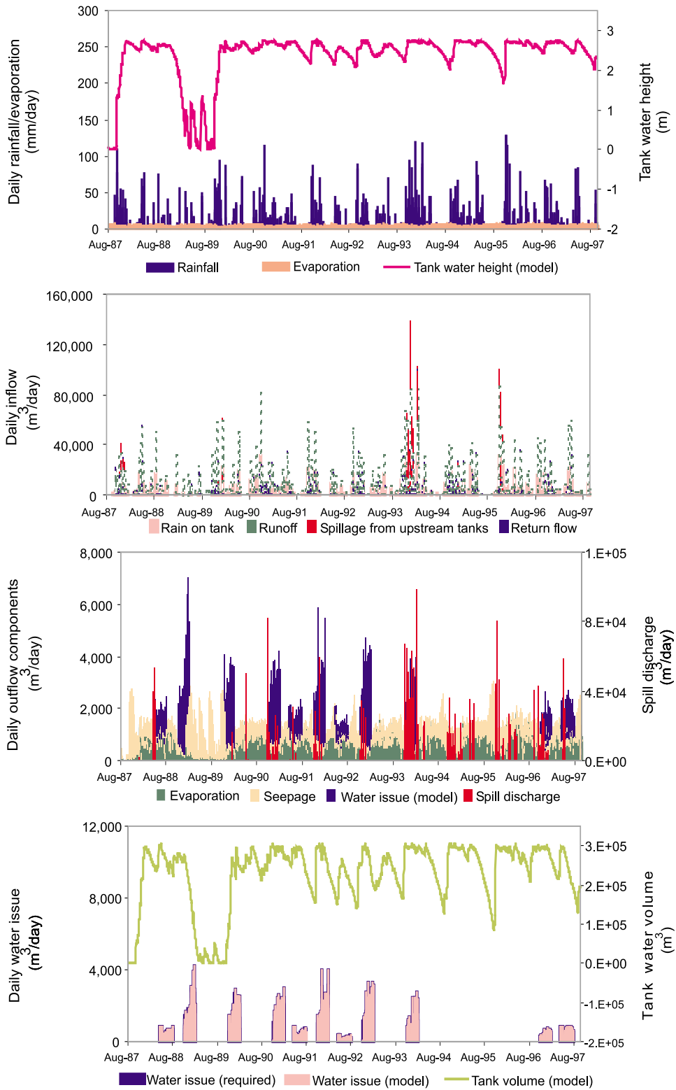
FIGURE 13. Predicted tank water height, volume and tank water balance components–Meegassagama.
