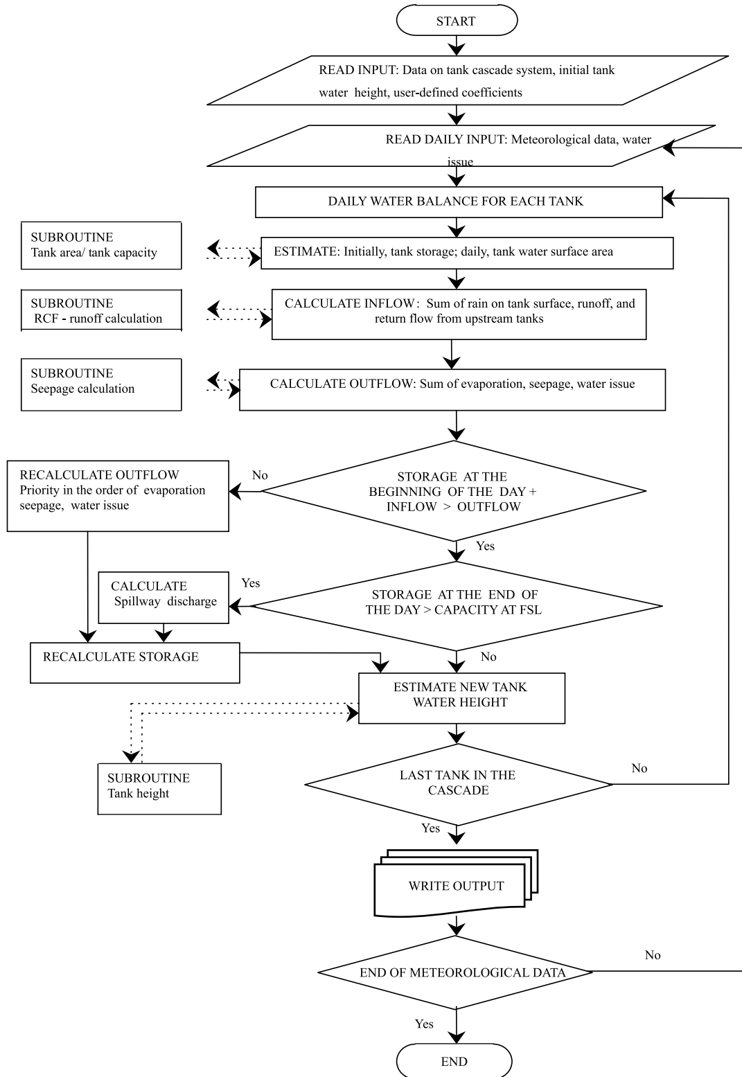
FIGURE 5. Flowchart of the Cascade model.
