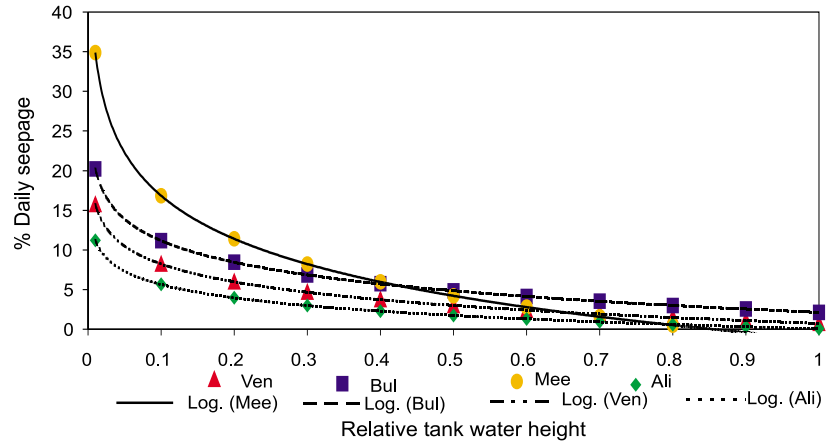
FIGURE A.2. Percent seepage as a function of the relative tank water height.
