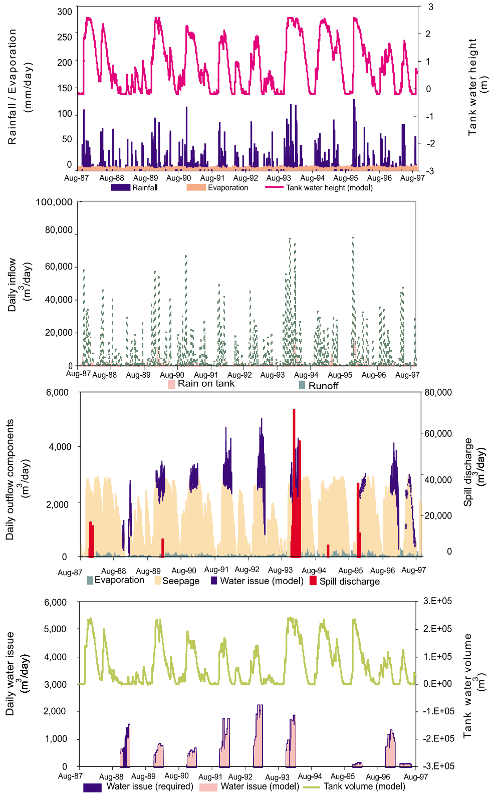
FIGURE 12. Predicted tank water height, volume, and tank water balance components–Bulankulama.
